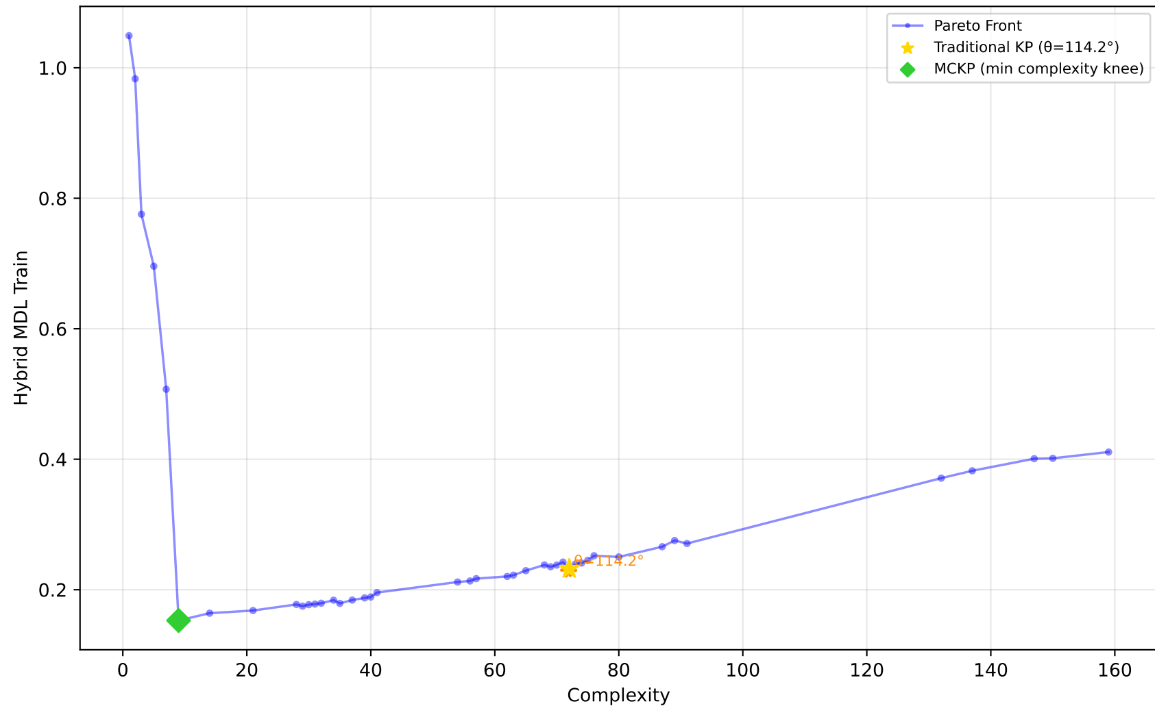
529_pollen - Run 27 - MVP - Hybrid MDL Train \lambda_1=0.90, \lambda_2=0.00, \lambda_3=0.00 | Difficulty: 1.00 | Method: hmr
