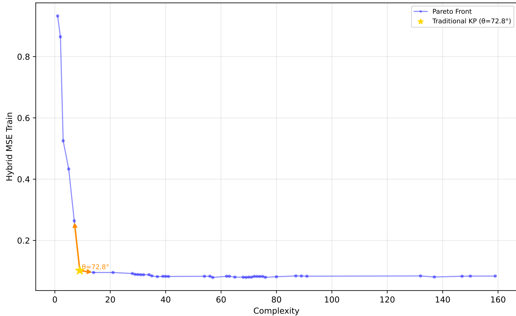
529_pollen - Run 27 - MVP - Hybrid MSE Train \lambda_1=0.00, \lambda_2=1.00, \lambda_3=0.80 | Difficulty: 1.00 | Method: hmr
