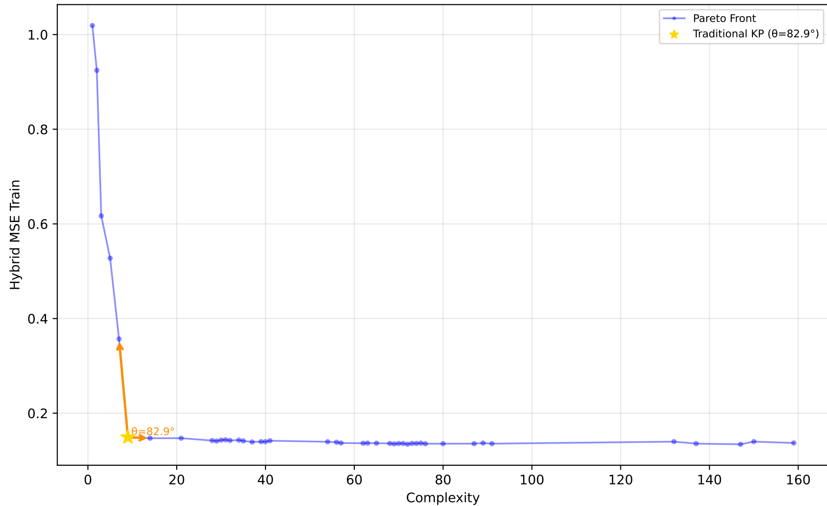
529_pollen - Run 27 - MVP - Hybrid MSE Train \lambda_1=0.90, \lambda_2=0.00, \lambda_3=0.00 | Difficulty: 1.00 | Method: hmr
