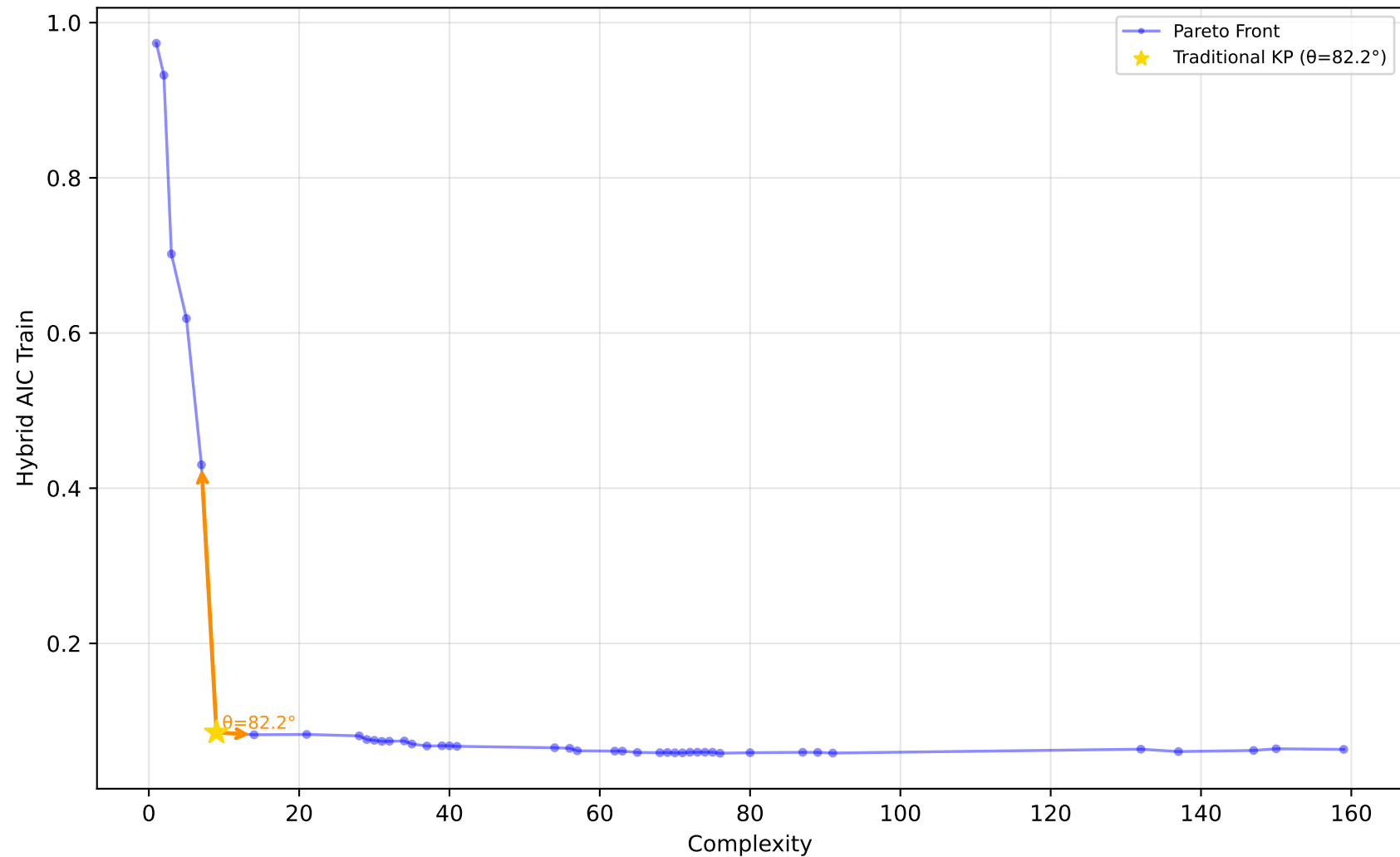
529_pollen - Run 27 - SVP - Hybrid AIC Train \lambda_1=0.10 , \lambda_2=0.80 , \lambda_3=0.30 | Difficulty: 1.00 | Method: hmr
