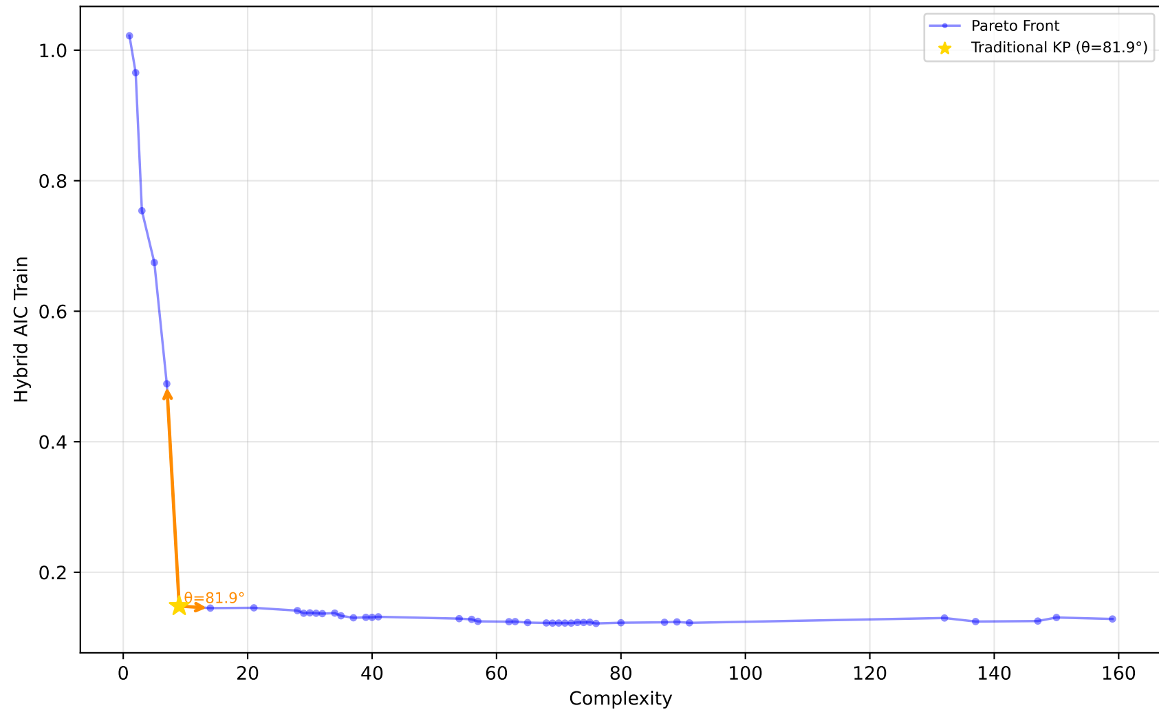
529_pollen - Run 27 - SVP - Hybrid AIC Train \lambda_1=0.60, \lambda_2=0.40, \lambda_3=1.00 | Difficulty: 1.00 | Method: hmr
