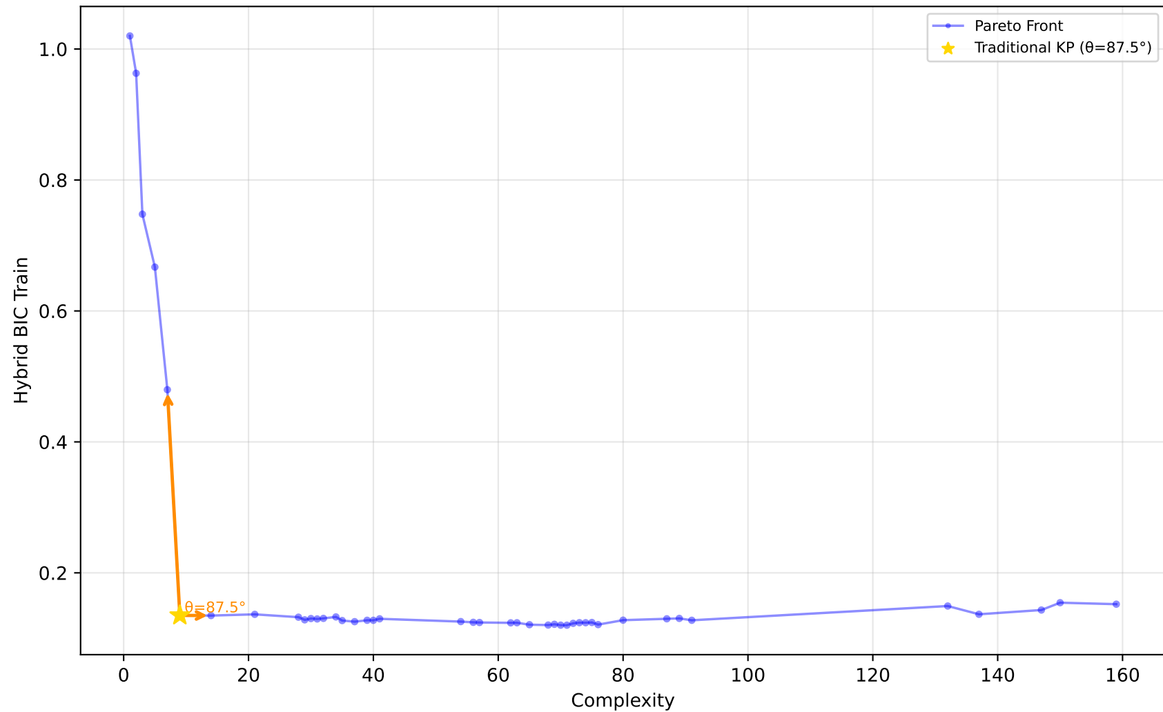
529_pollen - Run 27 - SVP - Hybrid BIC Train \lambda_1=0.60, \lambda_2=0.40, \lambda_3=1.00 | Difficulty: 1.00 | Method: hmr
