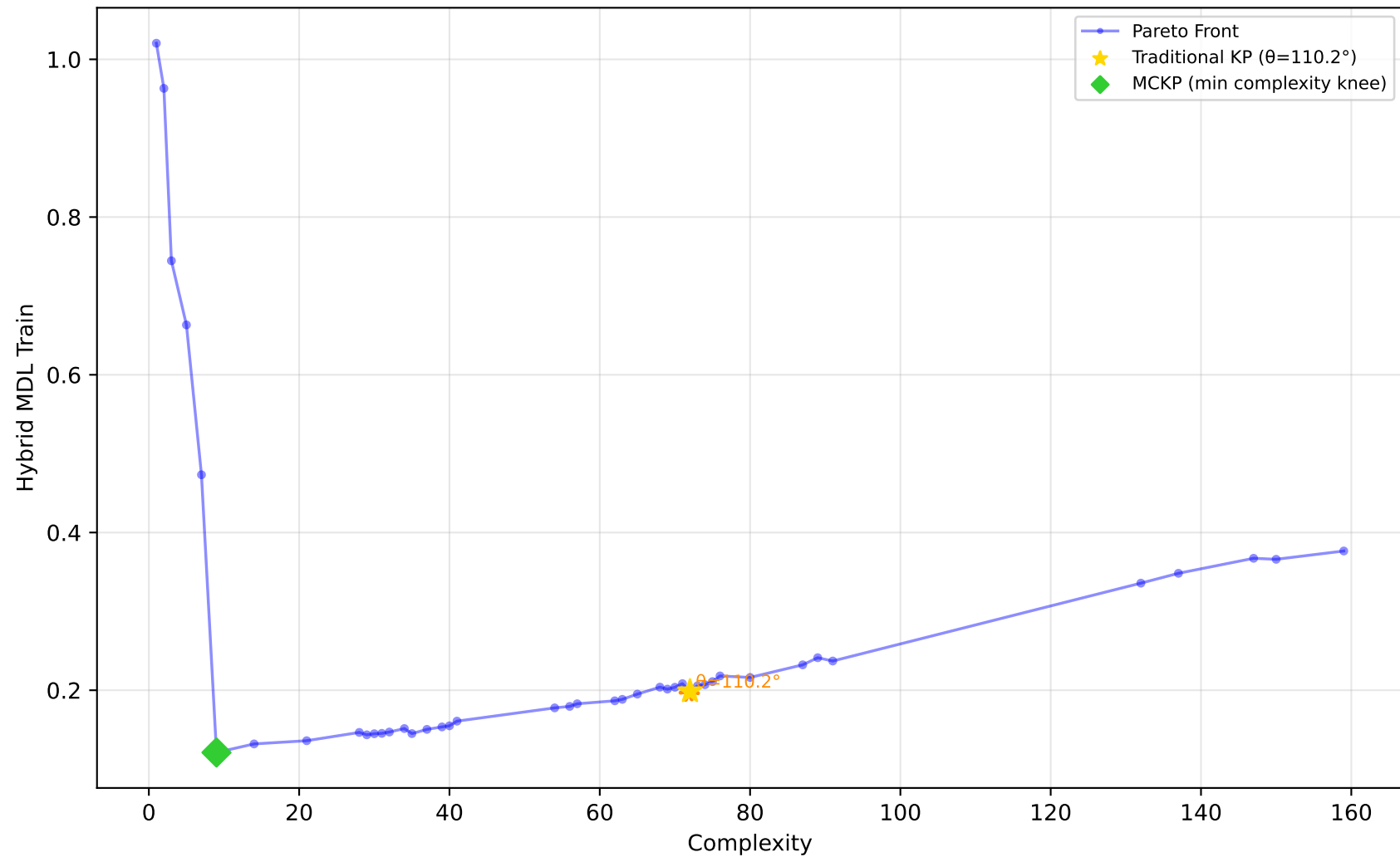
529_pollen - Run 27 - SVP - Hybrid MDL Train \lambda_1=0.60, \lambda_2=0.40, \lambda_3=1.00 | Difficulty: 1.00 | Method: hmr
