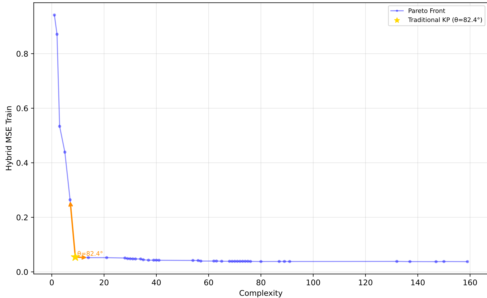
529_pollen - Run 27 - SVP - Hybrid MSE Train \lambda_1=0.10, \lambda_2=0.80, \lambda_3=0.30 | Difficulty: 1.00 | Method: hmr
