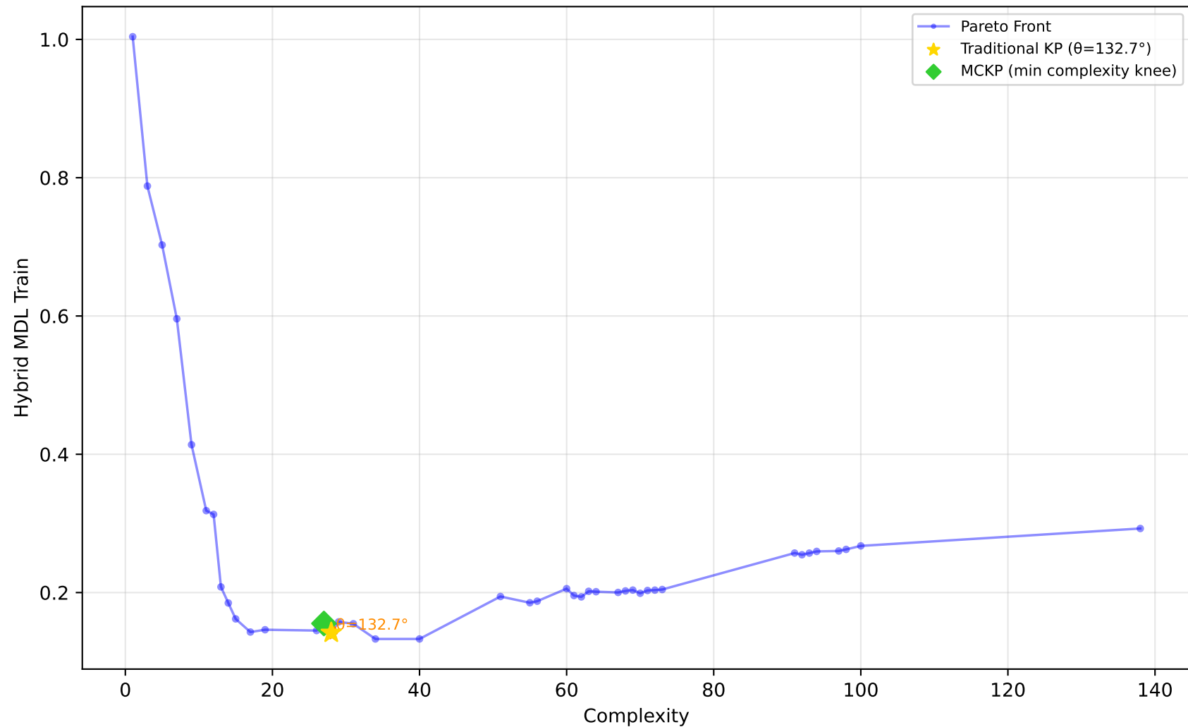
529_pollen - Run 28 - MVP - Hybrid MDL Train \lambda_1=0.90, \lambda_2=0.00, \lambda_3=0.00 | Difficulty: 1.00 | Method: hmr
