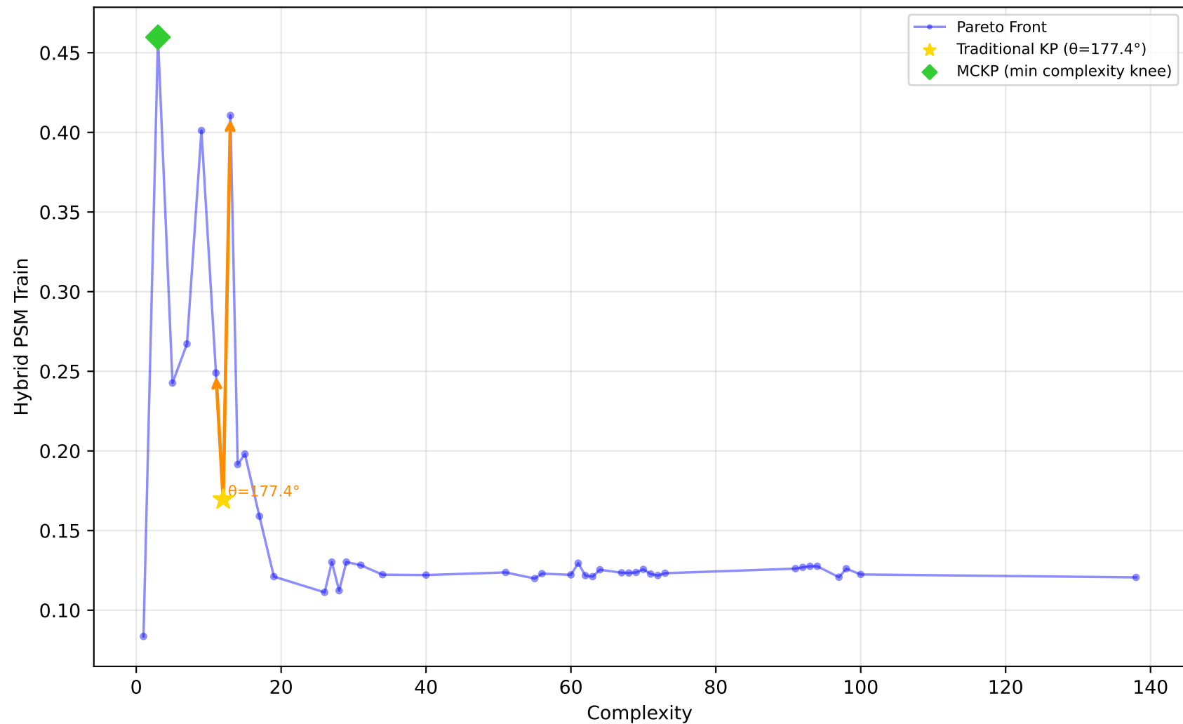
529_pollen - Run 28 - MVP - Hybrid PSM Train \lambda_1=0.90, \lambda_2=0.00, \lambda_3=0.00 | Difficulty: 1.00 | Method: hmr
