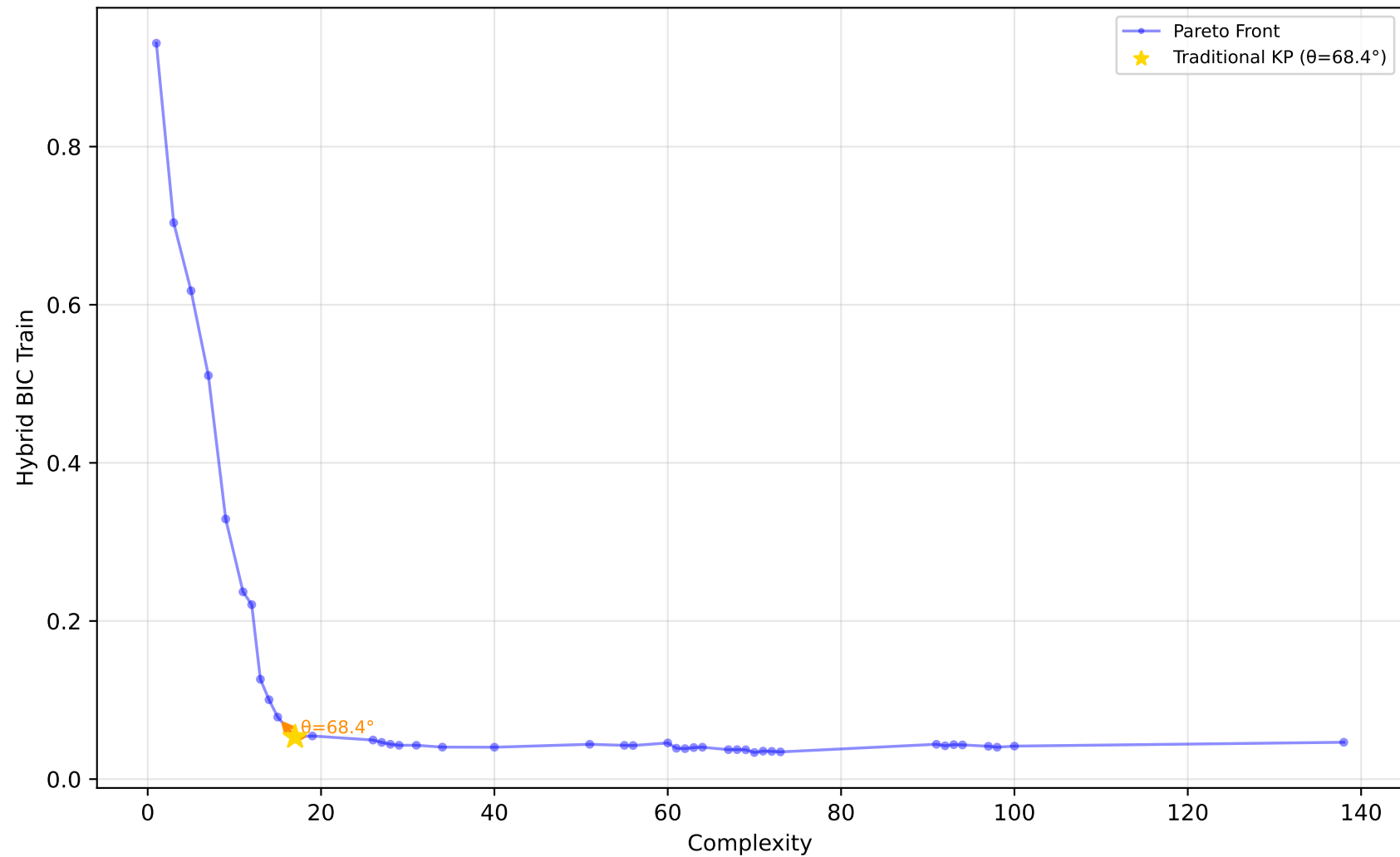
529_pollen - Run 28 - SVP - Hybrid BIC Train \lambda_1=0.10, \lambda_2=0.80, \lambda_3=0.30 | Difficulty: 1.00 | Method: hmr
