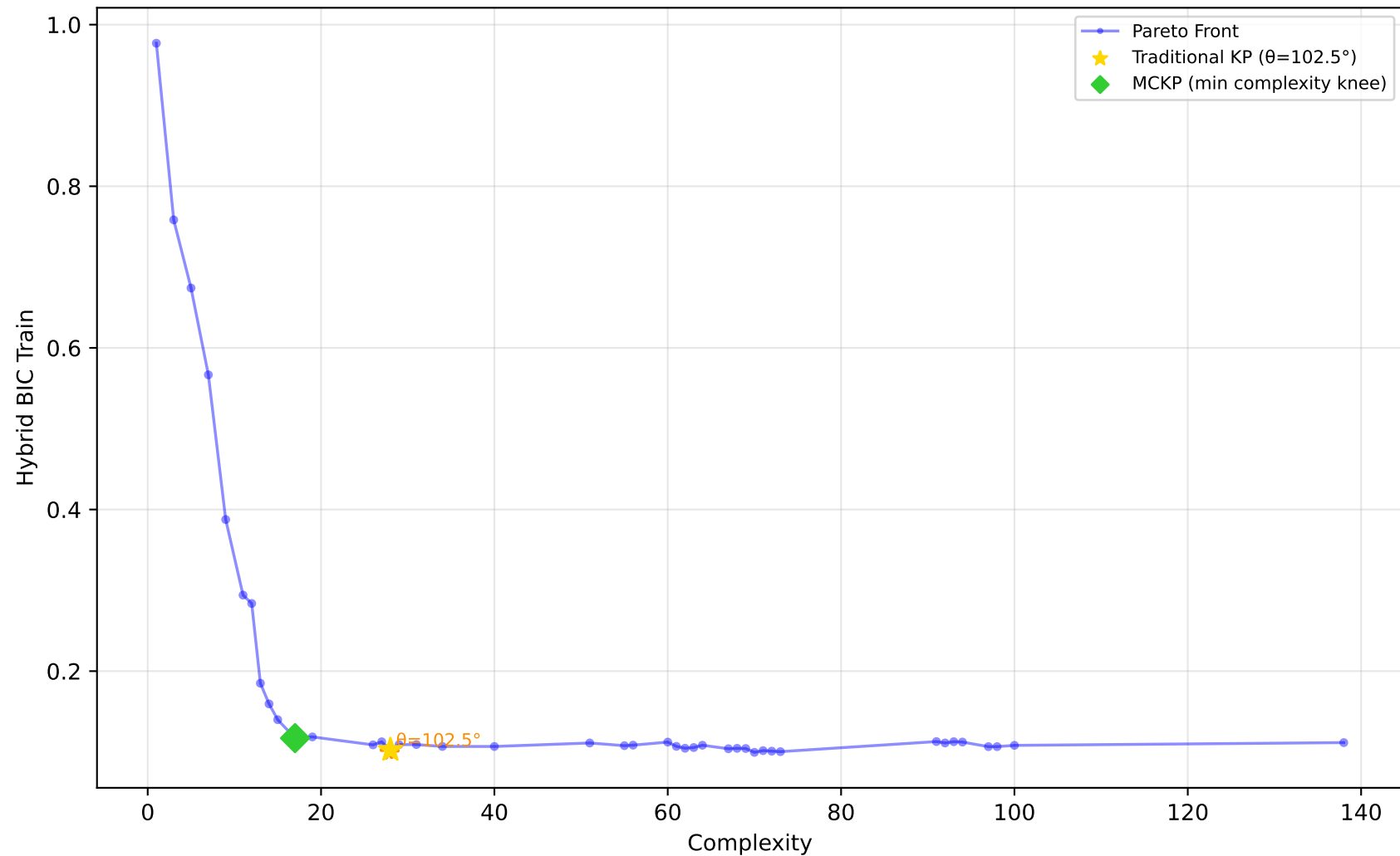
529_pollen - Run 28 - SVP - Hybrid BIC Train \lambda_1=0.60, \lambda_2=0.40, \lambda_3=1.00 | Difficulty: 1.00 | Method: hmr
