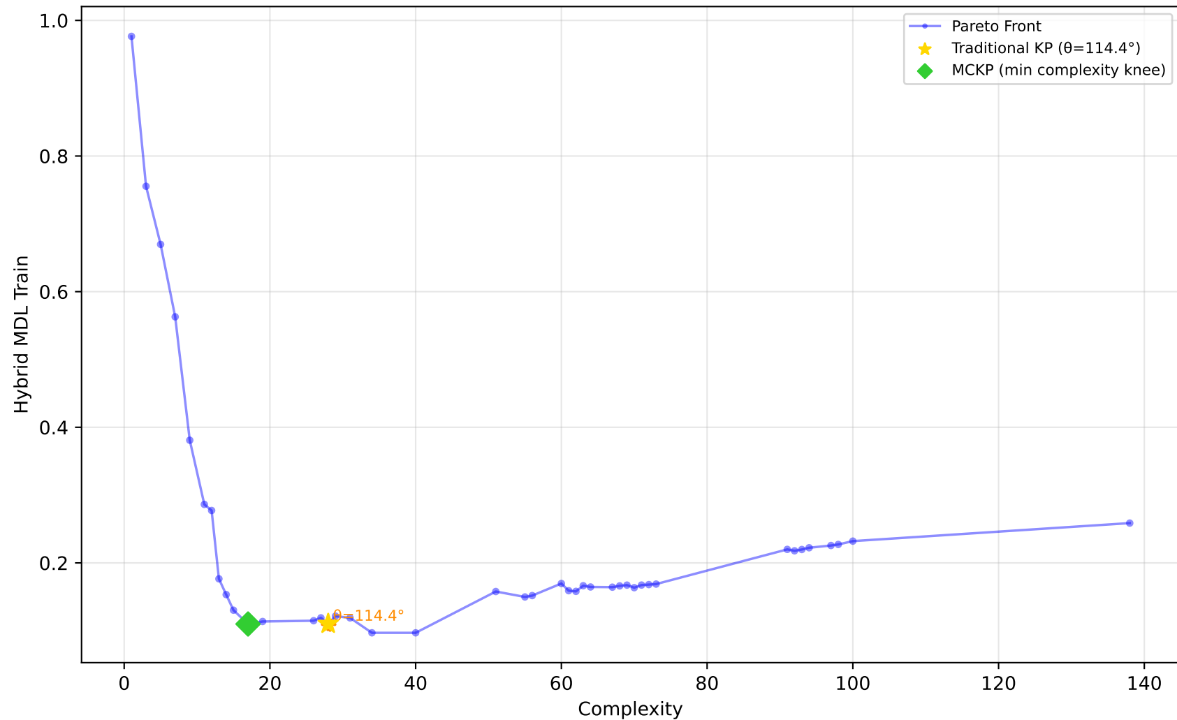
529_pollen - Run 28 - SVP - Hybrid MDL Train \lambda_1=0.60, \lambda_2=0.40, \lambda_3=1.00 | Difficulty: 1.00 | Method: hmr
