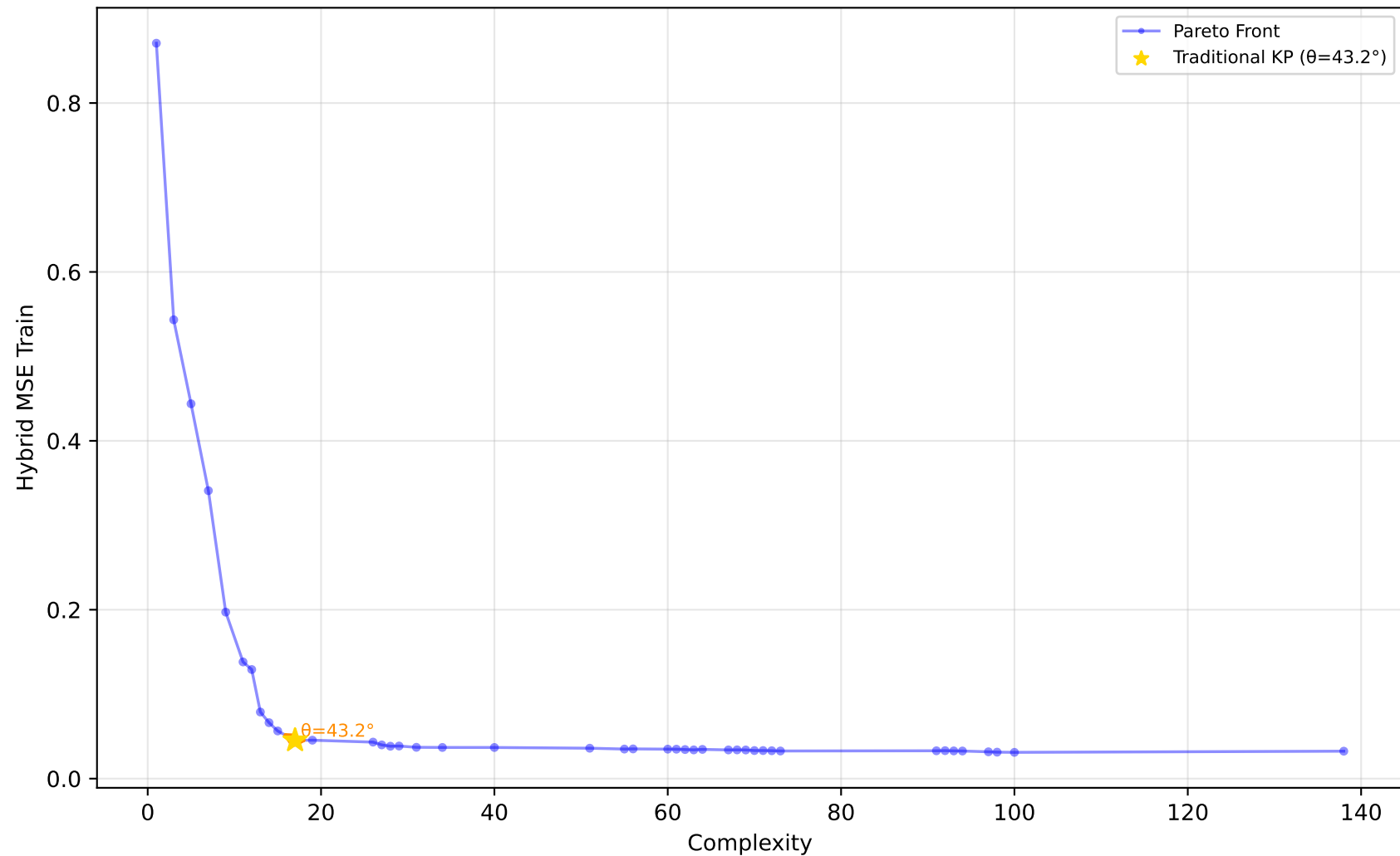
529_pollen - Run 28 - SVP - Hybrid MSE Train \lambda_1=0.10, \lambda_2=0.80, \lambda_3=0.30 | Difficulty: 1.00 | Method: hmr
