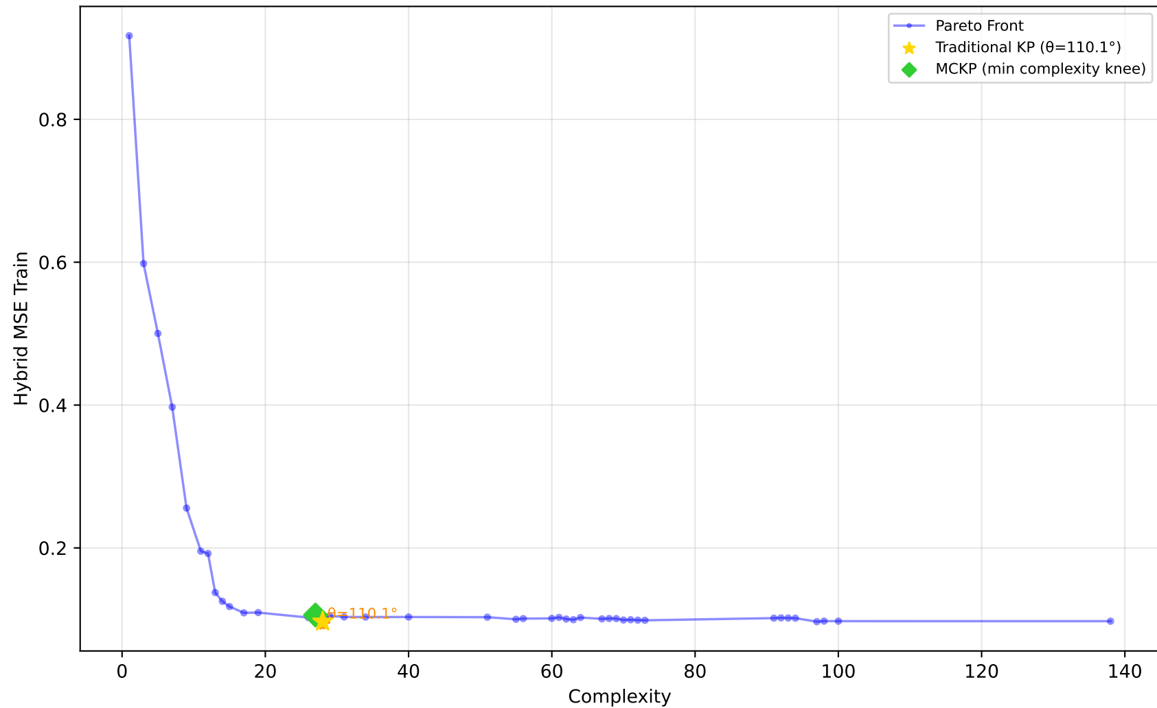
529_pollen - Run 28 - SVP - Hybrid MSE Train \lambda_1=0.60, \lambda_2=0.40, \lambda_3=1.00 | Difficulty: 1.00 | Method: hmr
