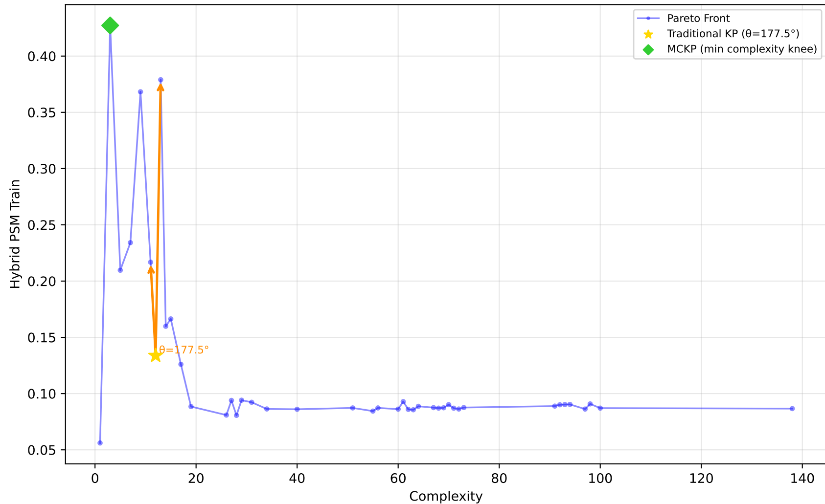
529_pollen - Run 28 - SVP - Hybrid PSM Train \lambda_1=0.60, \lambda_2=0.40, \lambda_3=1.00 | Difficulty: 1.00 | Method: hmr
