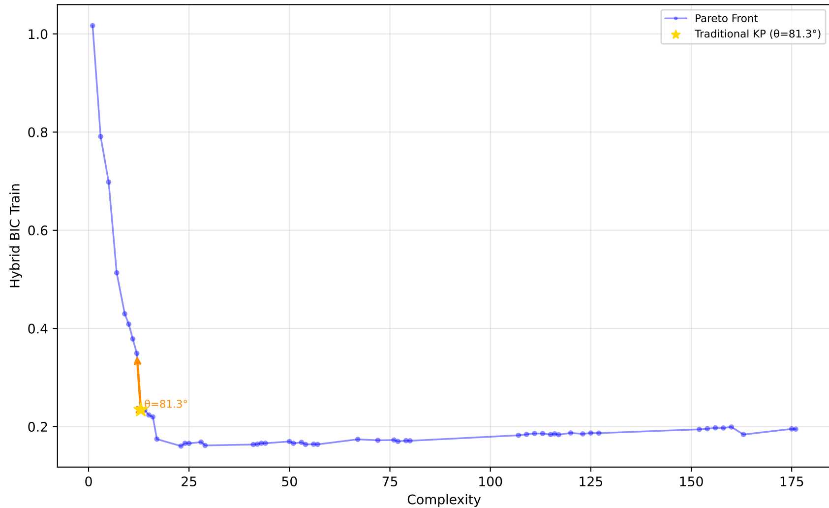
529_pollen - Run 29 - MVP - Hybrid BIC Train \lambda_1=0.90, \lambda_2=0.00, \lambda_3=0.00 | Difficulty: 1.00 | Method: hmr
