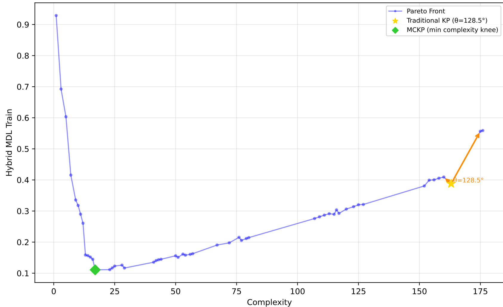
529_pollen - Run 29 - MVP - Hybrid MDL Train \lambda_1=0.00, \lambda_2=1.00, \lambda_3=0.80 | Difficulty: 1.00 | Method: hmr
