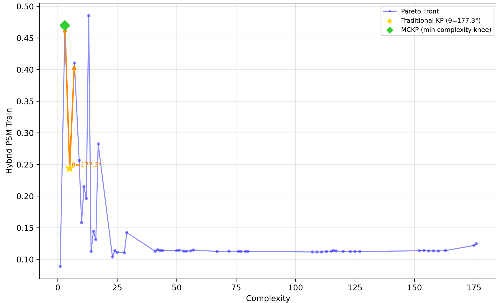
529_pollen - Run 29 - MVP - Hybrid PSM Train \lambda_1=0.90, \lambda_2=0.00, \lambda_3=0.00 | Difficulty: 1.00 | Method: hmr
