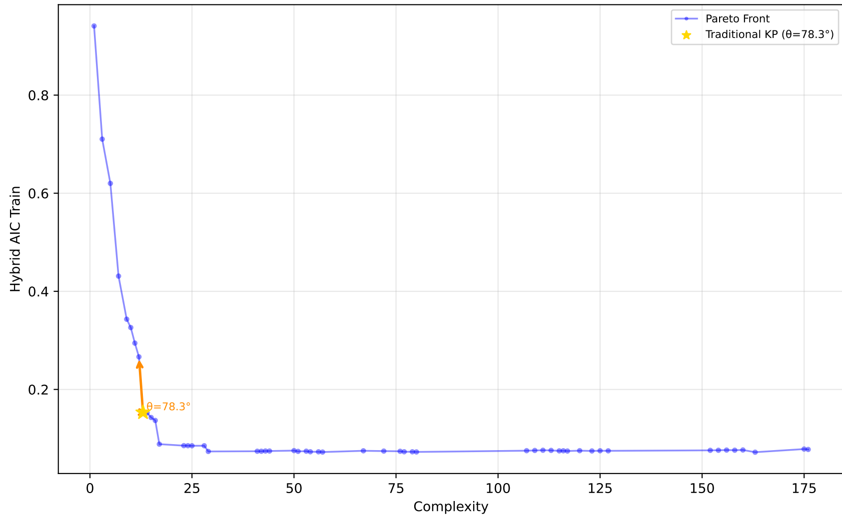
529_pollen - Run 29 - SVP - Hybrid AIC Train \lambda_1=0.10 , \lambda_2=0.80 , \lambda_3=0.30 | Difficulty: 1.00 | Method: hmr
