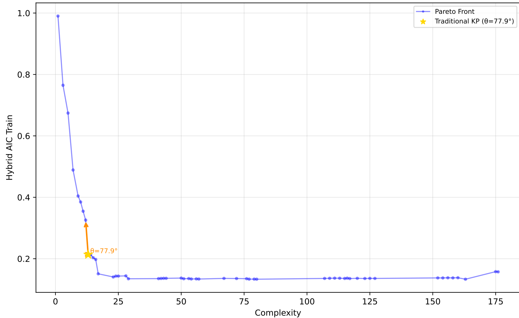
529_pollen - Run 29 - SVP - Hybrid AIC Train \lambda_1=0.60, \lambda_2=0.40, \lambda_3=1.00 | Difficulty: 1.00 | Method: hmr
