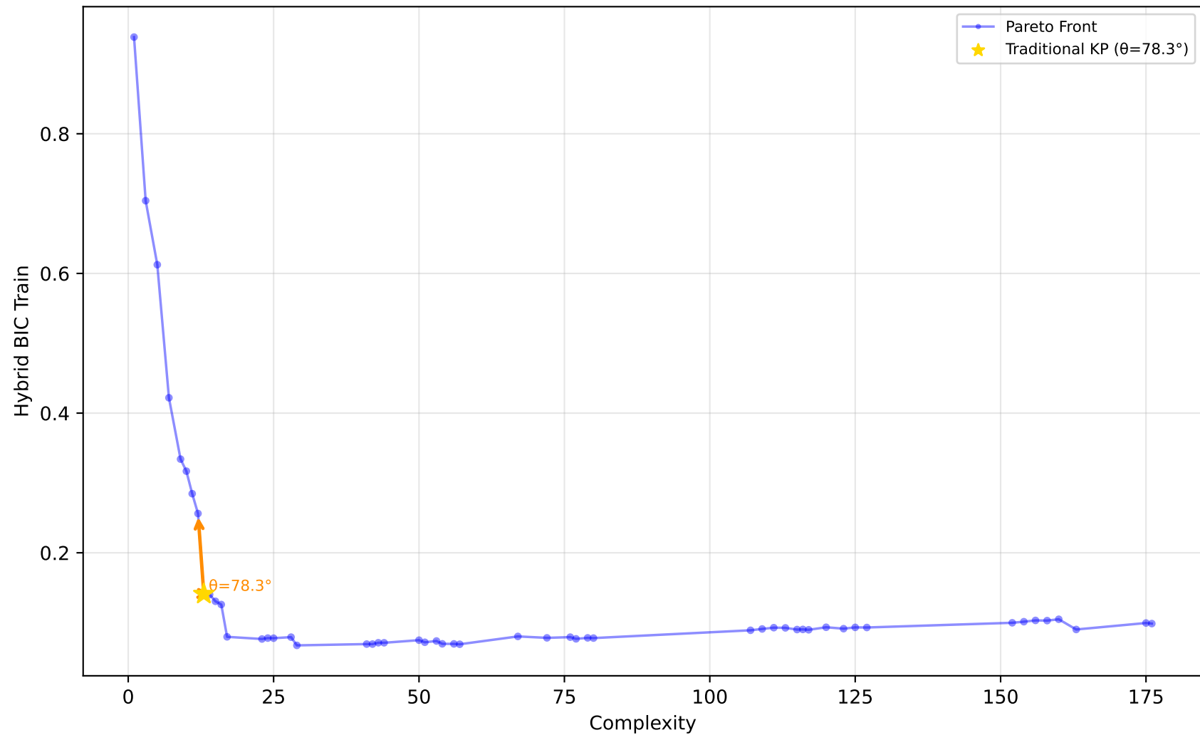
529_pollen - Run 29 - SVP - Hybrid BIC Train \lambda_1=0.10, \lambda_2=0.80, \lambda_3=0.30 | Difficulty: 1.00 | Method: hmr
