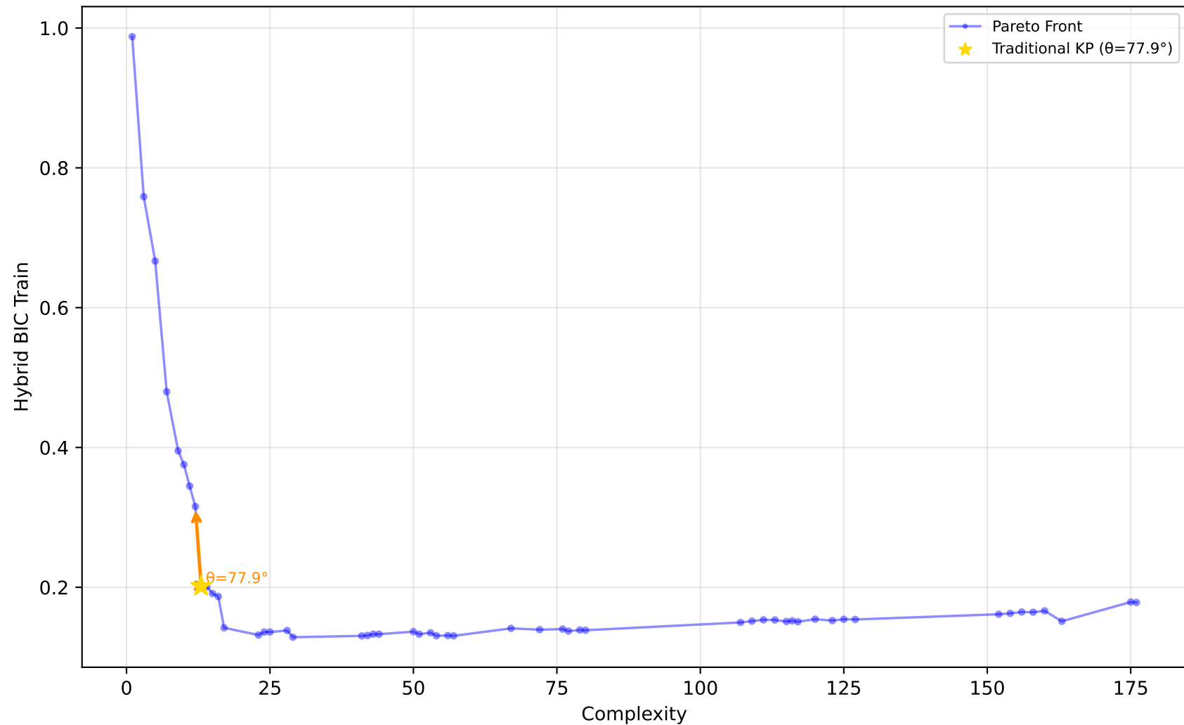
529_pollen - Run 29 - SVP - Hybrid BIC Train \lambda_1=0.60, \lambda_2=0.40, \lambda_3=1.00 | Difficulty: 1.00 | Method: hmr
