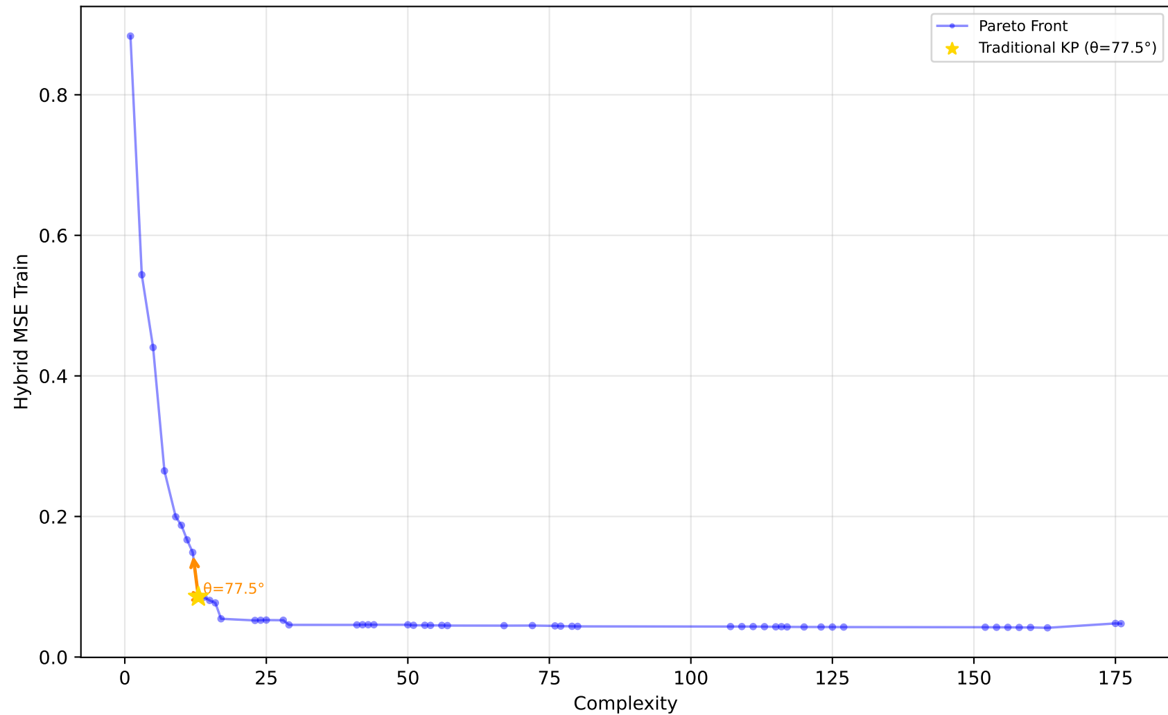
529_pollen - Run 29 - SVP - Hybrid MSE Train \lambda_1=0.10, \lambda_2=0.80, \lambda_3=0.30 | Difficulty: 1.00 | Method: hmr
