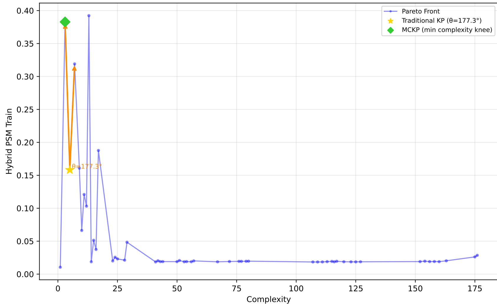
529_pollen - Run 29 - SVP - Hybrid PSM Train \lambda_1=0.10, \lambda_2=0.80, \lambda_3=0.30 | Difficulty: 1.00 | Method: hmr
