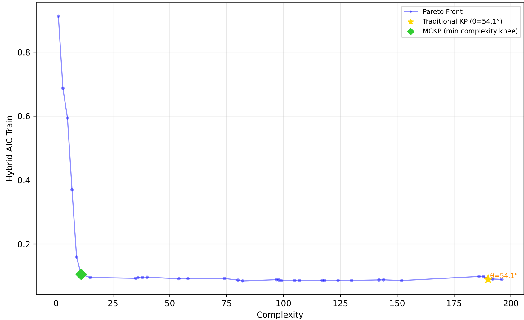
529_pollen - Run 2 - MVP - Hybrid AIC Train \lambda_1=0.00 , \lambda_2=1.00 , \lambda_3=0.80 | Difficulty: 1.00 | Method: hmr
