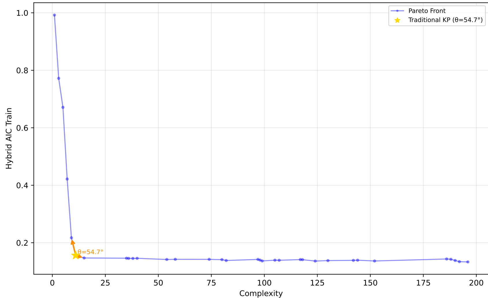
529_pollen - Run 2 - MVP - Hybrid AIC Train \lambda_1=0.90, \lambda_2=0.00, \lambda_3=0.00 | Difficulty: 1.00 | Method: hmr
