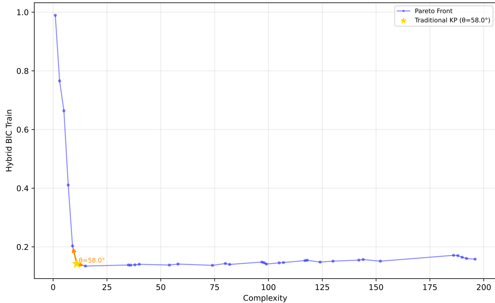
529_pollen - Run 2 - MVP - Hybrid BIC Train \lambda_1=0.90, \lambda_2=0.00, \lambda_3=0.00 | Difficulty: 1.00 | Method: hmr
