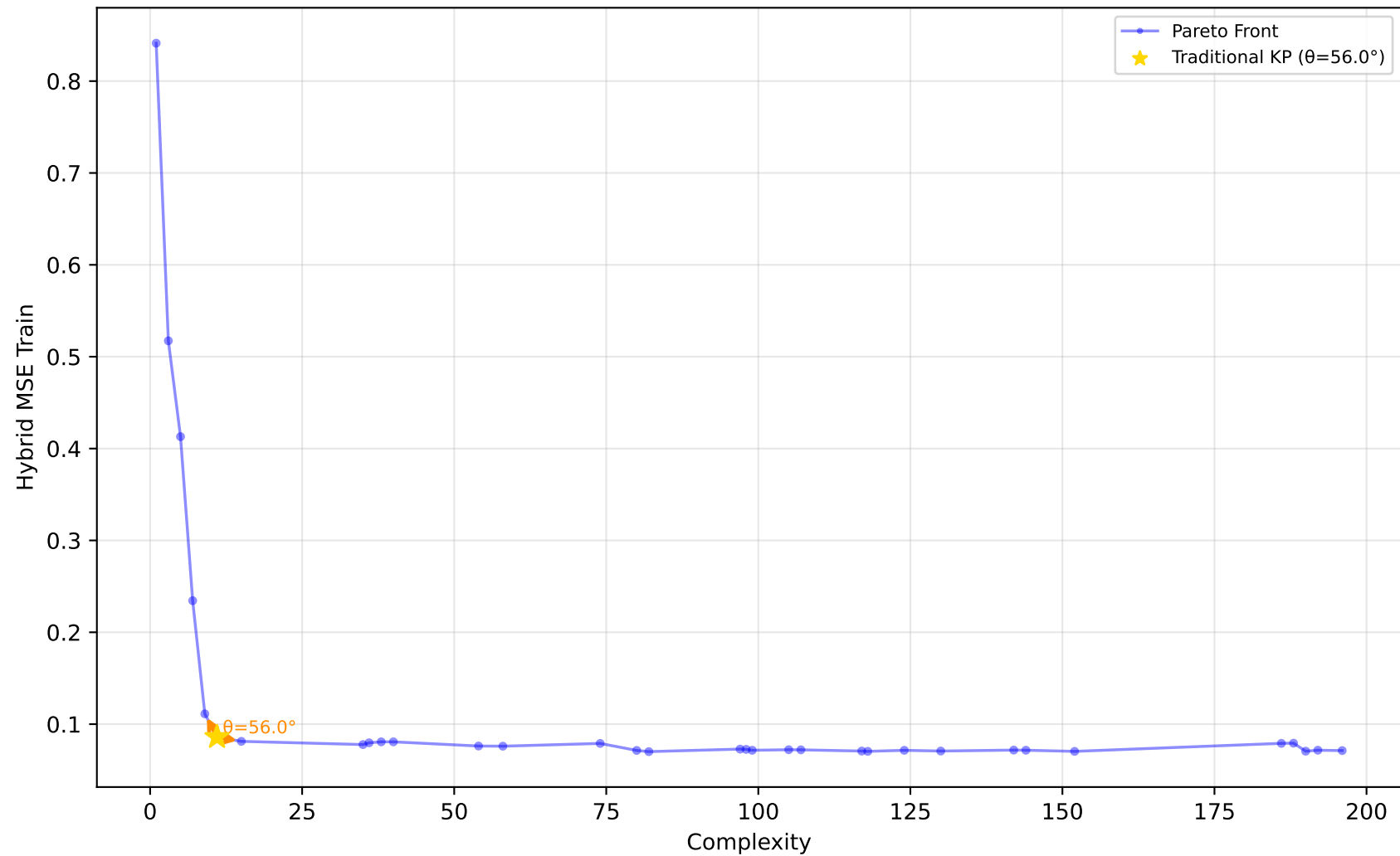
529_pollen - Run 2 - MVP - Hybrid MSE Train \lambda_1=0.00, \lambda_2=1.00, \lambda_3=0.80 | Difficulty: 1.00 | Method: hmr
