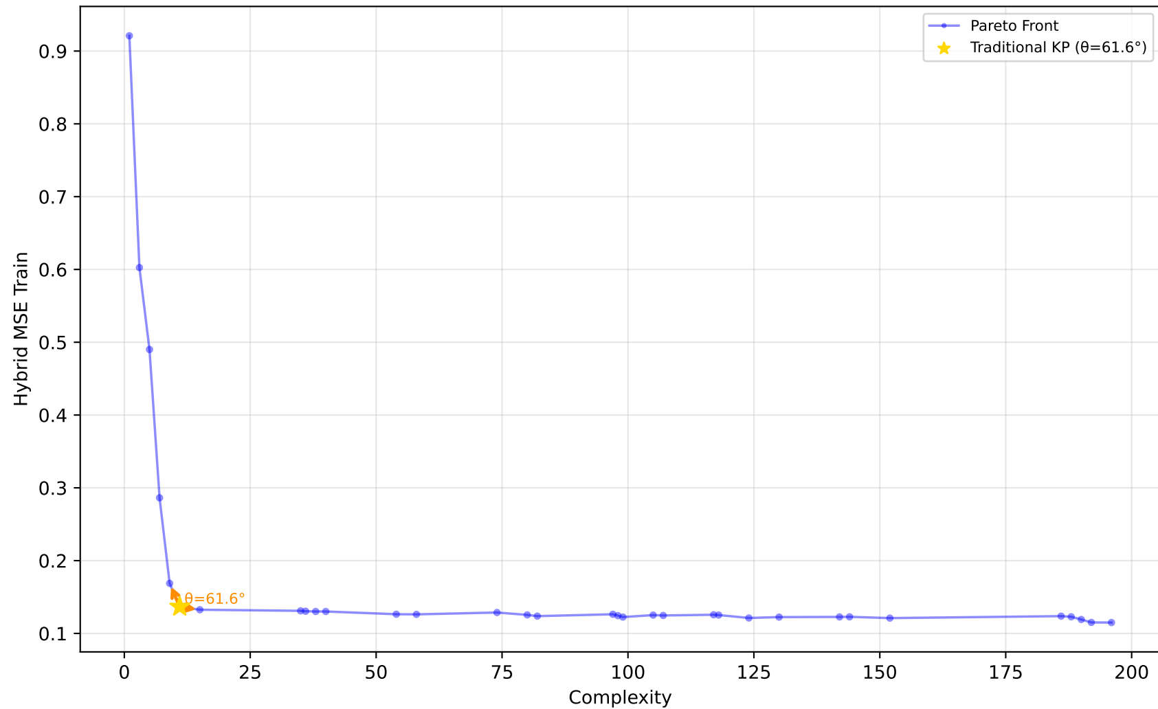
529_pollen - Run 2 - MVP - Hybrid MSE Train \lambda_1=0.90, \lambda_2=0.00, \lambda_3=0.00 | Difficulty: 1.00 | Method: hmr
