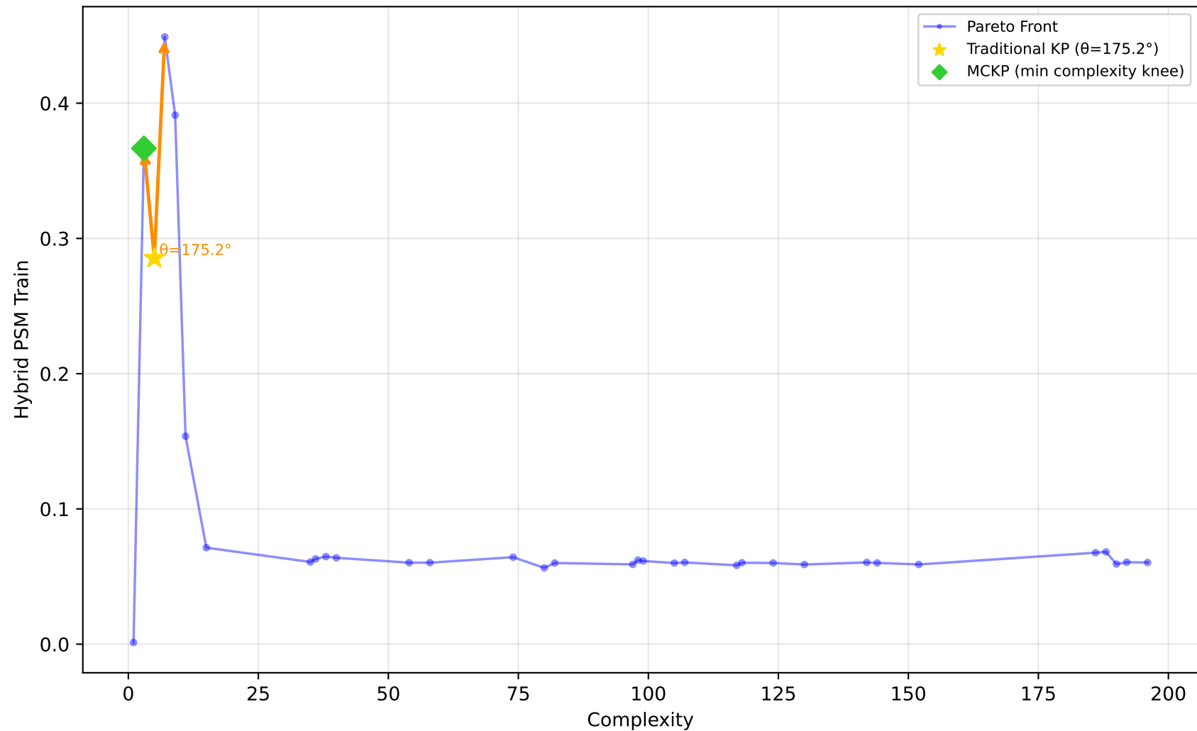
529_pollen - Run 2 - MVP - Hybrid PSM Train \lambda_1=0.00, \lambda_2=1.00, \lambda_3=0.80 | Difficulty: 1.00 | Method: hmr
