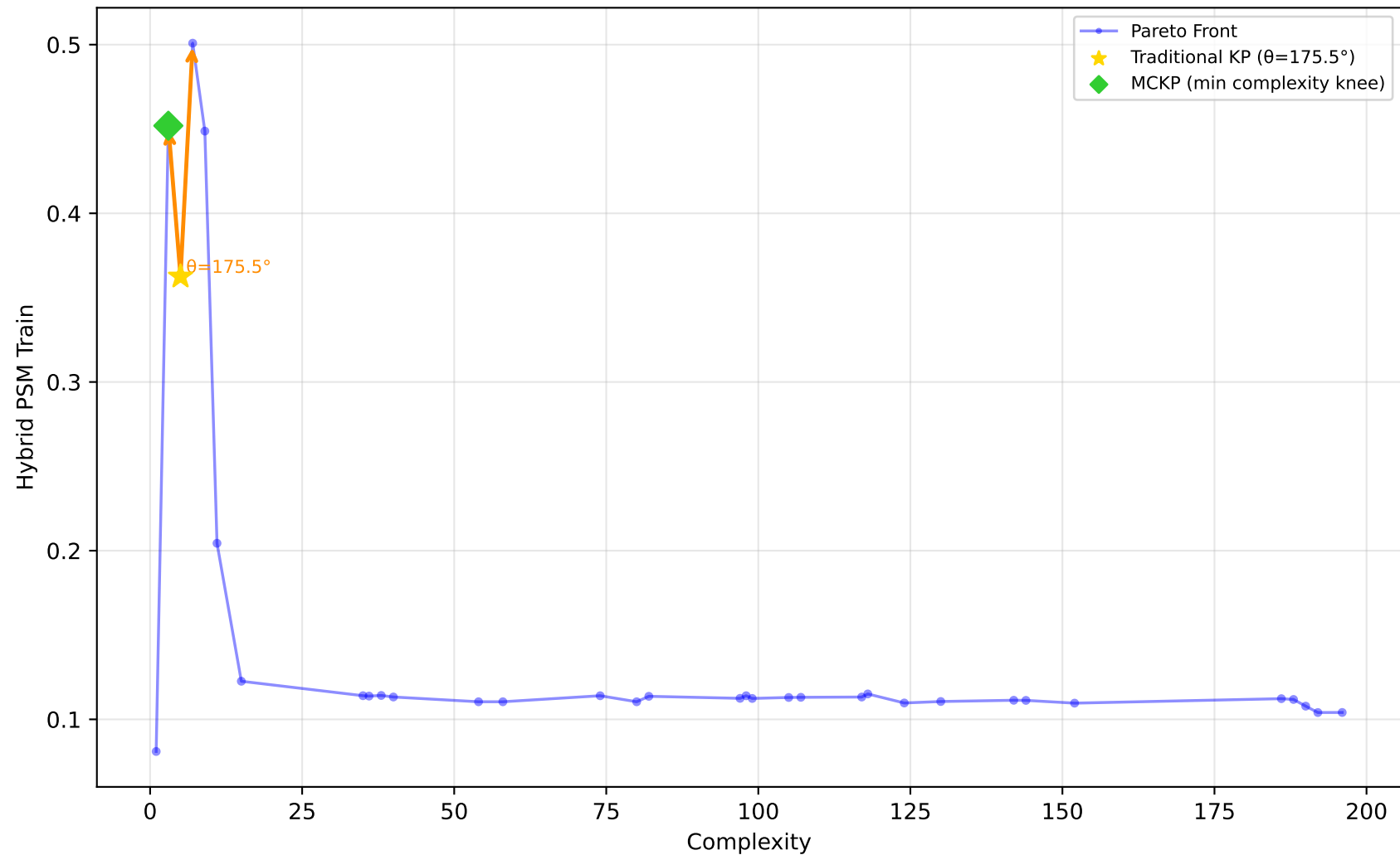
529_pollen - Run 2 - MVP - Hybrid PSM Train \lambda_1=0.90, \lambda_2=0.00, \lambda_3=0.00 | Difficulty: 1.00 | Method: hmr
