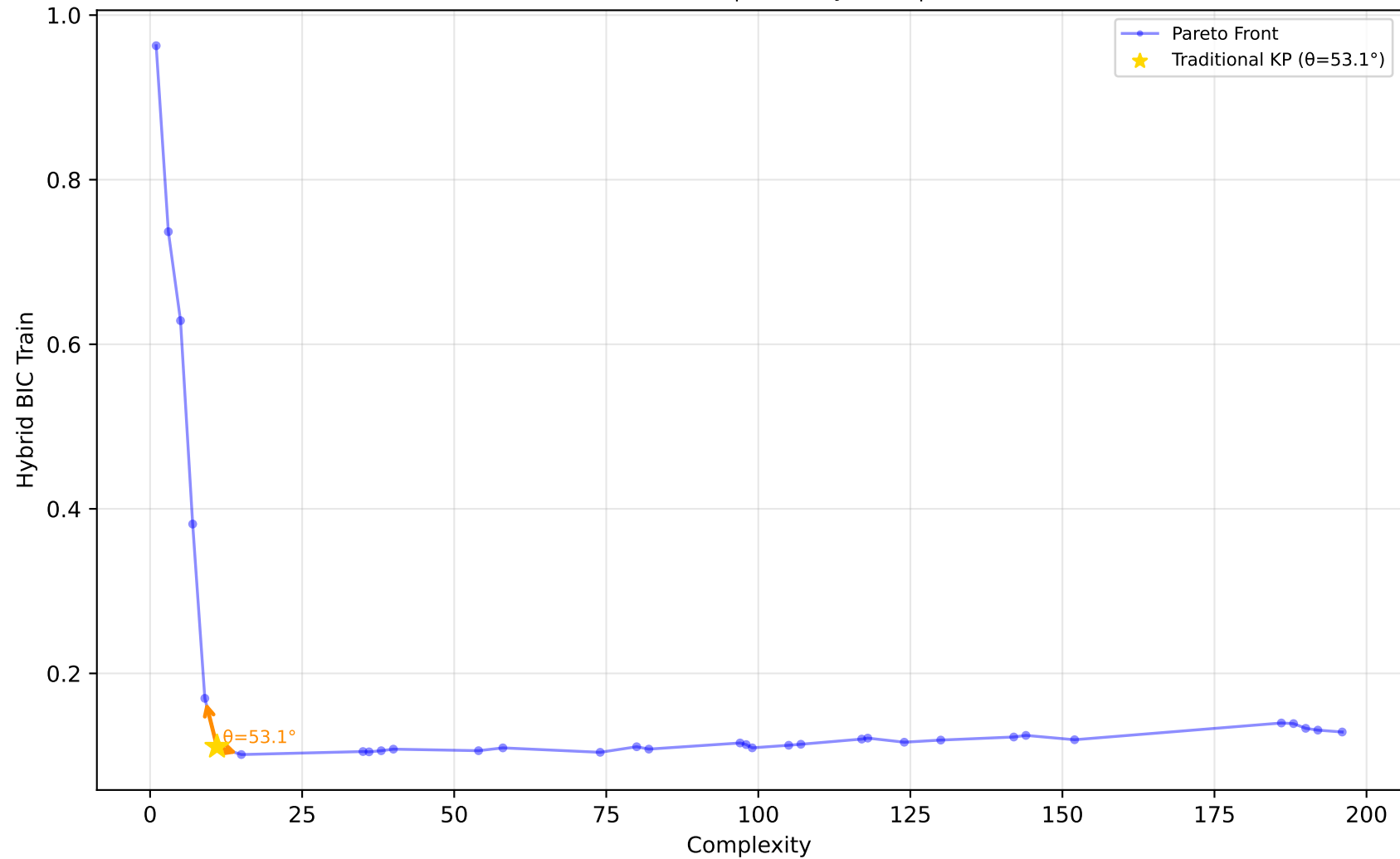
529_pollen - Run 2 - SVP - Hybrid BIC Train \lambda_1=0.60, \lambda_2=0.40, \lambda_3=1.00 | Difficulty: 1.00 | Method: hmr
