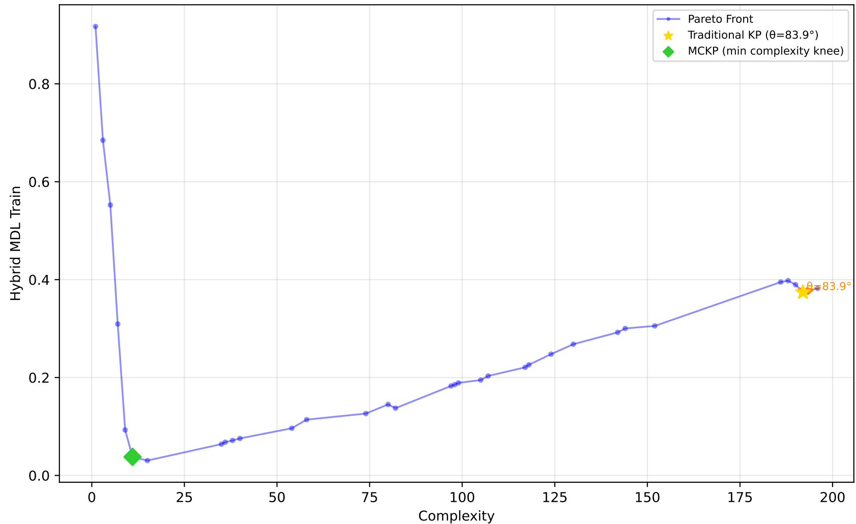
529_pollen - Run 2 - SVP - Hybrid MDL Train \lambda_1=0.10, \lambda_2=0.80, \lambda_3=0.30 | Difficulty: 1.00 | Method: hmr
