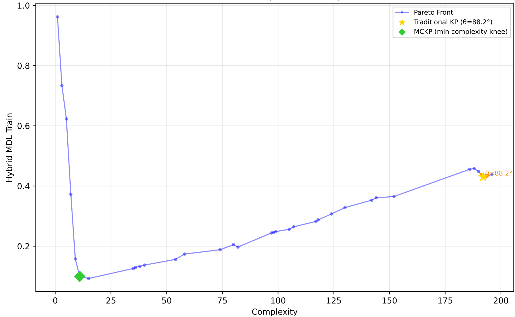
529_pollen - Run 2 - SVP - Hybrid MDL Train \lambda_1=0.60, \lambda_2=0.40, \lambda_3=1.00 | Difficulty: 1.00 | Method: hmr
