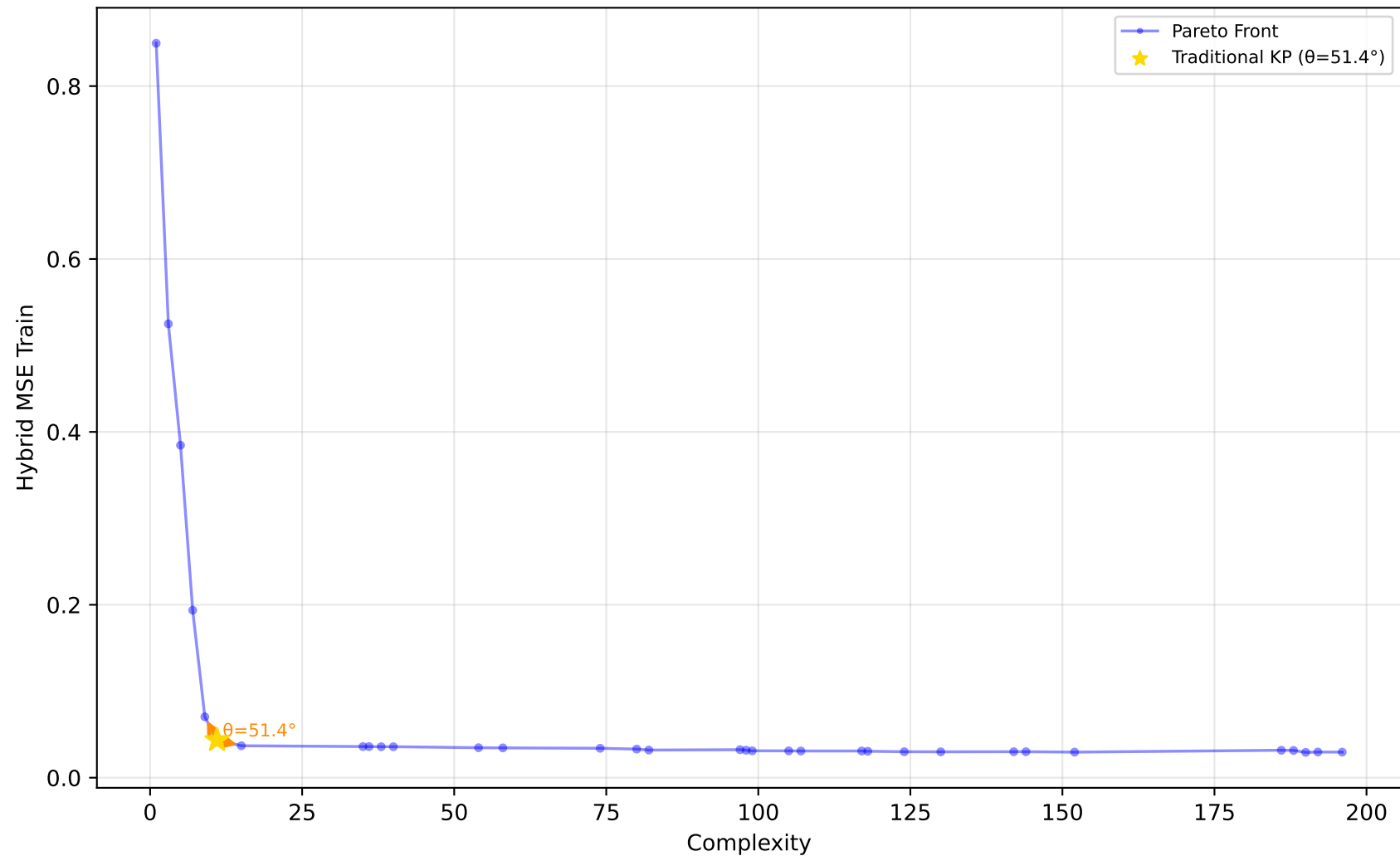
529_pollen - Run 2 - SVP - Hybrid MSE Train \lambda_1=0.10, \lambda_2=0.80, \lambda_3=0.30 | Difficulty: 1.00 | Method: hmr
