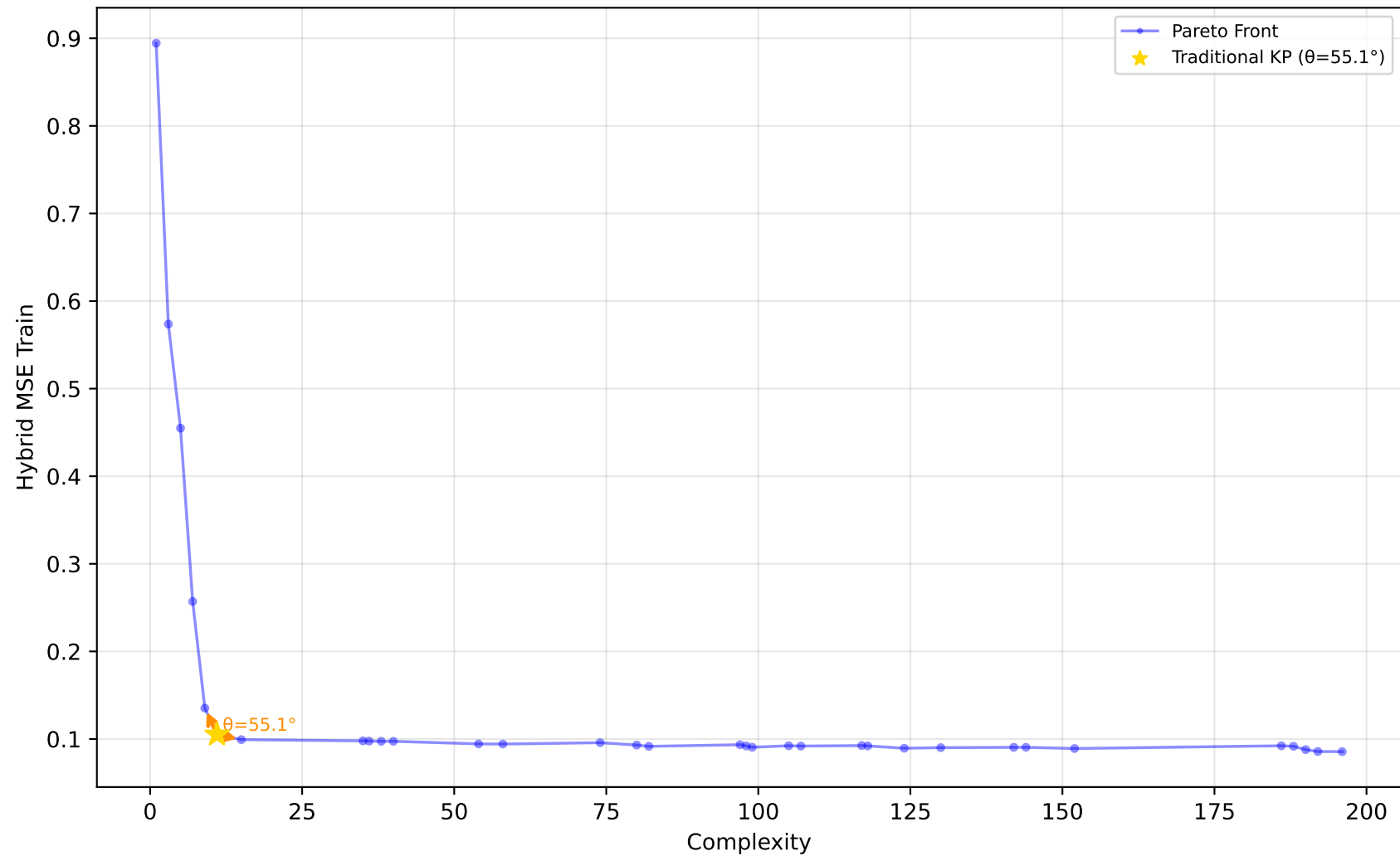
529_pollen - Run 2 - SVP - Hybrid MSE Train \lambda_1=0.60, \lambda_2=0.40, \lambda_3=1.00 | Difficulty: 1.00 | Method: hmr
