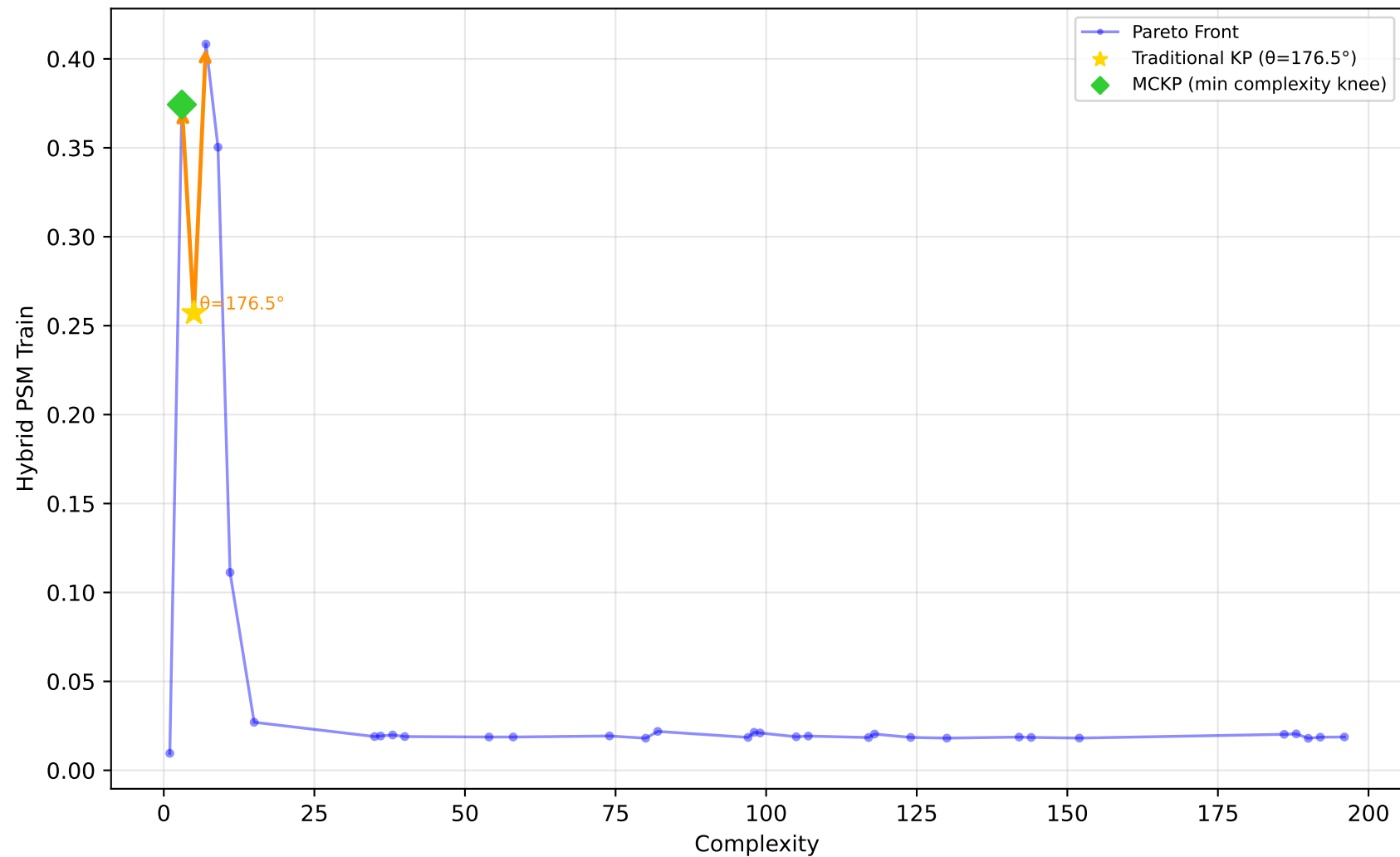
529_pollen - Run 2 - SVP - Hybrid PSM Train \lambda_1=0.10, \lambda_2=0.80, \lambda_3=0.30 | Difficulty: 1.00 | Method: hmr
