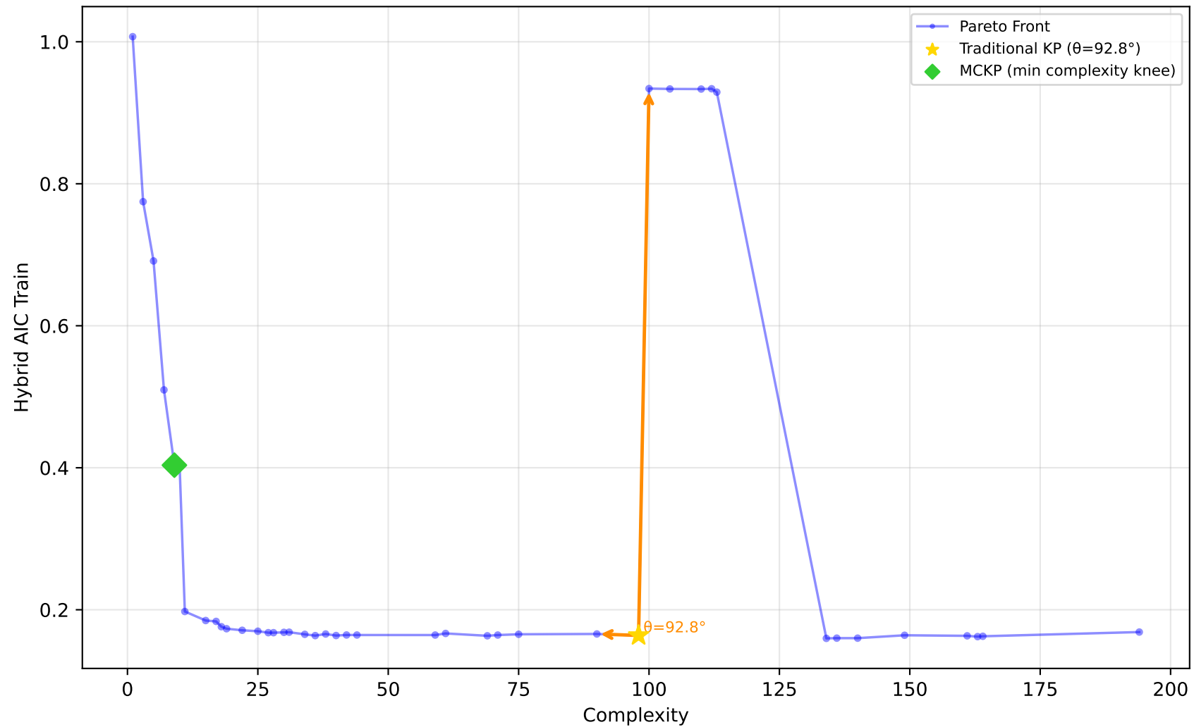
529_pollen - Run 30 - MVP - Hybrid AIC Train \lambda_1=0.90, \lambda_2=0.00, \lambda_3=0.00 | Difficulty: 1.00 | Method: hmr
