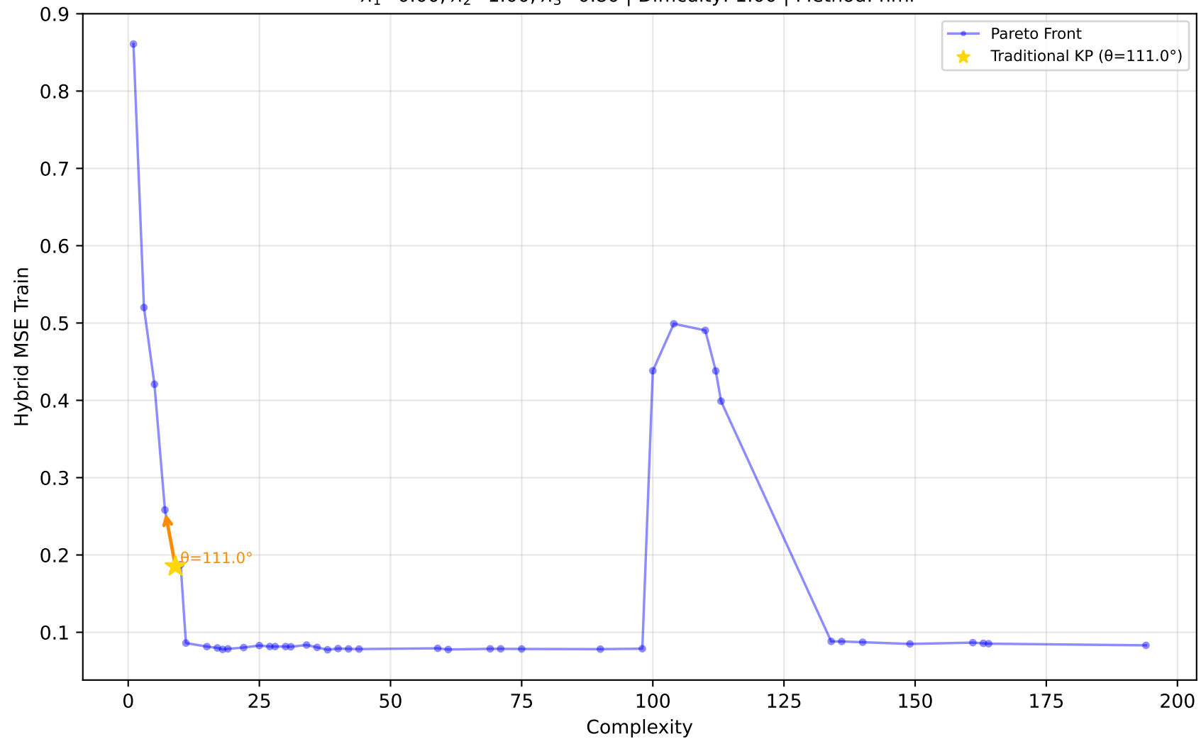
529_pollen - Run 30 - MVP - Hybrid MSE Train \lambda_1=0.00, \lambda_2=1.00, \lambda_3=0.80 | Difficulty: 1.00 | Method: hmr
