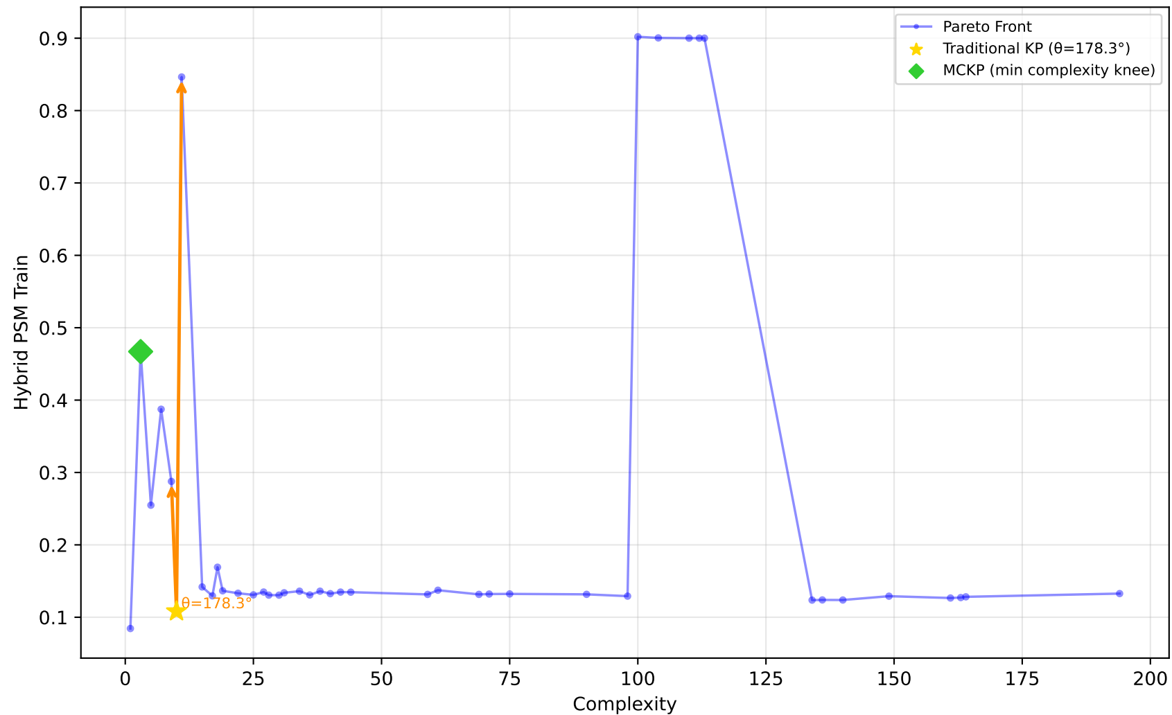
529_pollen - Run 30 - MVP - Hybrid PSM Train \lambda_1=0.90, \lambda_2=0.00, \lambda_3=0.00 | Difficulty: 1.00 | Method: hmr
