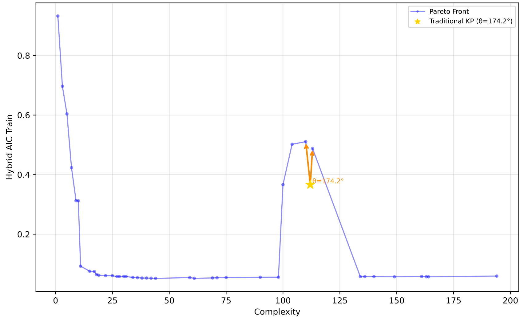
529_pollen - Run 30 - SVP - Hybrid AIC Train \lambda_1=0.10 , \lambda_2=0.80 , \lambda_3=0.30 | Difficulty: 1.00 | Method: hmr
