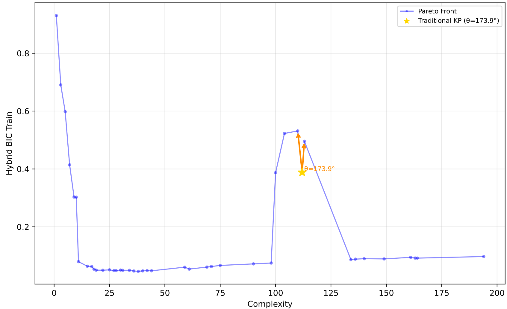
529_pollen - Run 30 - SVP - Hybrid BIC Train \lambda_1=0.10, \lambda_2=0.80, \lambda_3=0.30 | Difficulty: 1.00 | Method: hmr
