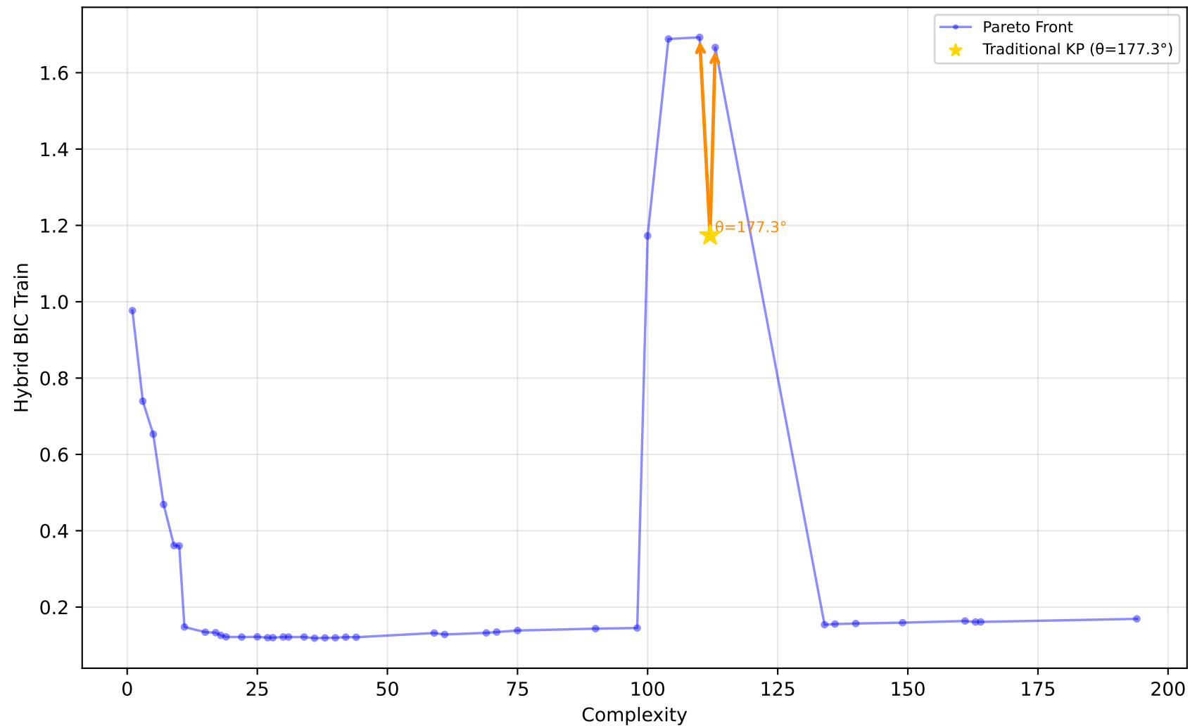
529_pollen - Run 30 - SVP - Hybrid BIC Train \lambda_1=0.60, \lambda_2=0.40, \lambda_3=1.00 | Difficulty: 1.00 | Method: hmr
