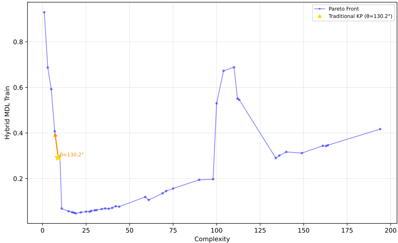
529_pollen - Run 30 - SVP - Hybrid MDL Train \lambda_1=0.10 , \lambda_2=0.80 , \lambda_3=0.30 | Difficulty: 1.00 | Method: hmr
