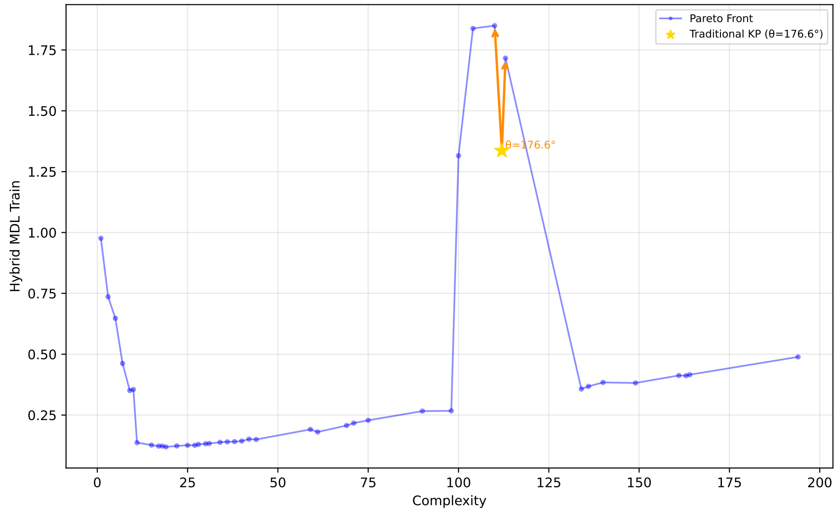
529_pollen - Run 30 - SVP - Hybrid MDL Train \lambda_1=0.60, \lambda_2=0.40, \lambda_3=1.00 | Difficulty: 1.00 | Method: hmr
