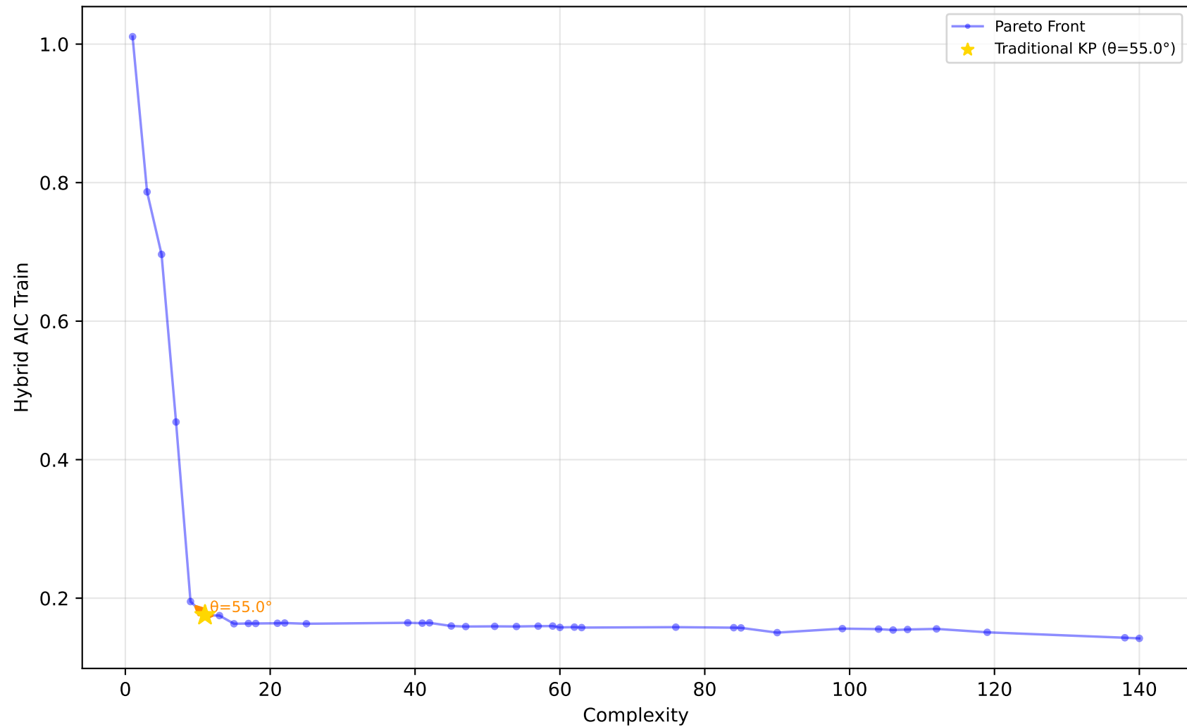
529_pollen - Run 3 - MVP - Hybrid AIC Train \lambda_1=0.90, \lambda_2=0.00, \lambda_3=0.00 | Difficulty: 1.00 | Method: hmr
