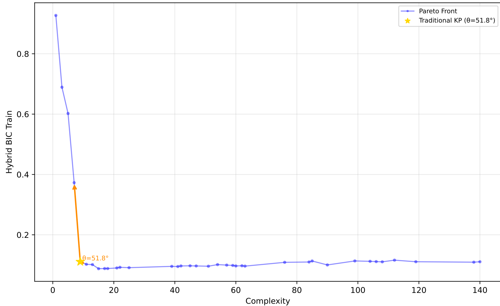
529_pollen - Run 3 - MVP - Hybrid BIC Train \lambda_1=0.00, \lambda_2=1.00, \lambda_3=0.80 | Difficulty: 1.00 | Method: hmr
