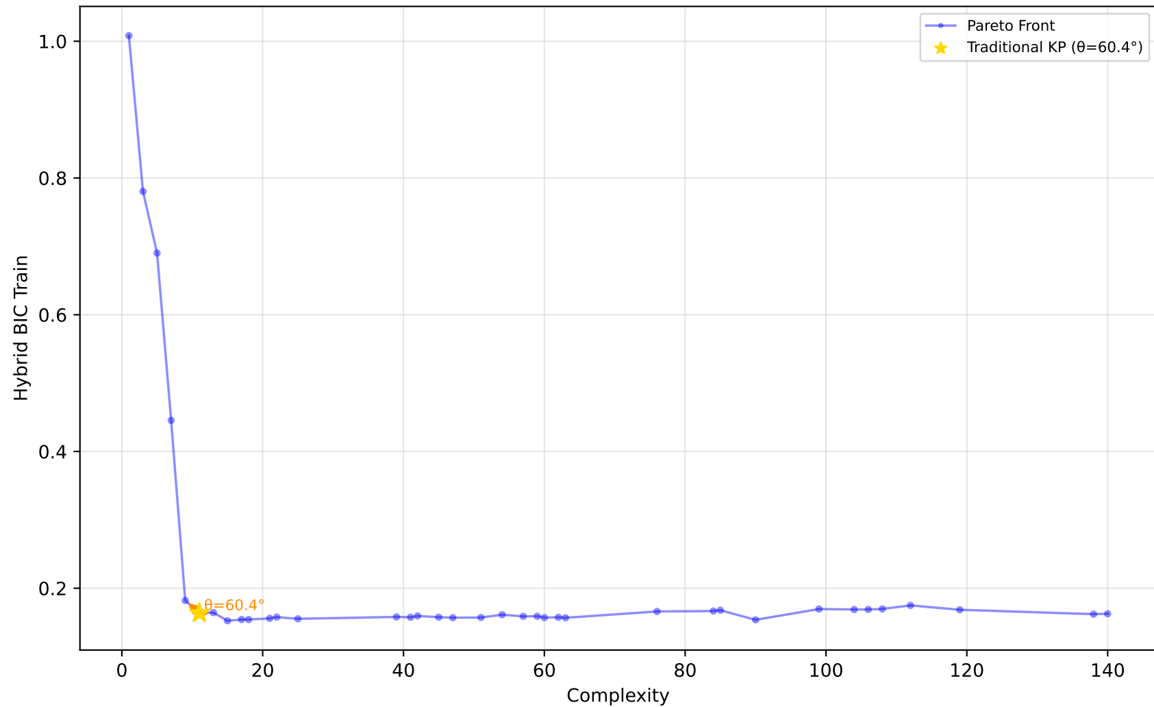
529_pollen - Run 3 - MVP - Hybrid BIC Train \lambda_1=0.90, \lambda_2=0.00, \lambda_3=0.00 | Difficulty: 1.00 | Method: hmr
