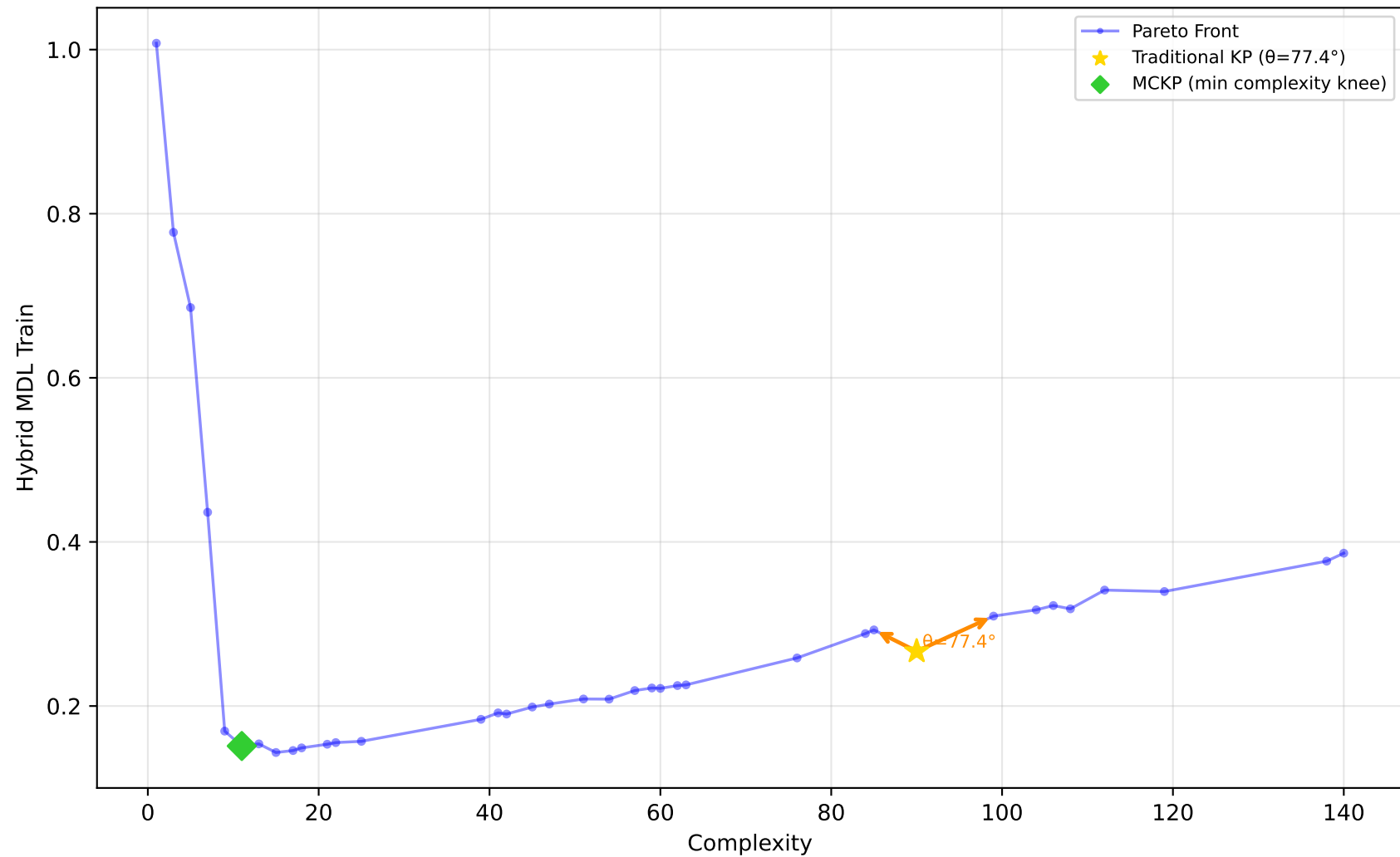
529_pollen - Run 3 - MVP - Hybrid MDL Train \lambda_1=0.90, \lambda_2=0.00, \lambda_3=0.00 | Difficulty: 1.00 | Method: hmr
